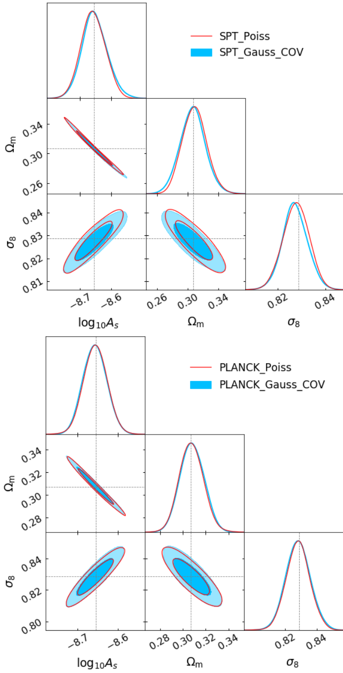
Fig. B.2. Contour plots at 68 and 95 per cent of confidence level for the Poissonian (red) and Gaussian (blue) likelihood for the SPT-like ( top ) and Planck-like ( bottom ) samples. The grey dotted lines represent the input values of parameters.
