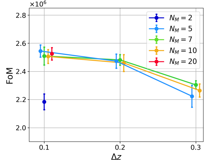
Fig. 6. Same as Fig. 5, for the Gaussian likelihood.
