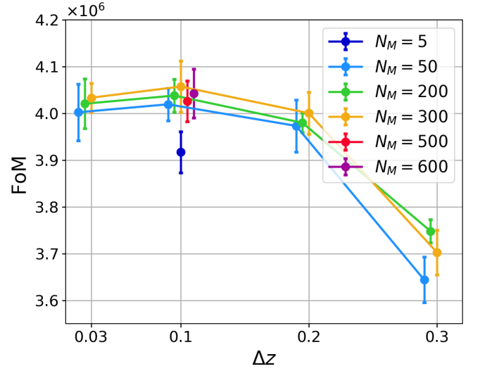
Fig. 5. Figure of merit for the Poissonian likelihood as a function of the redshift bin widths, for different numbers of mass bins. The points represent the average value over 5 realizations and the error bars are the standard error of the mean. A small horizontal offset has been applied to make the comparison clearer.
