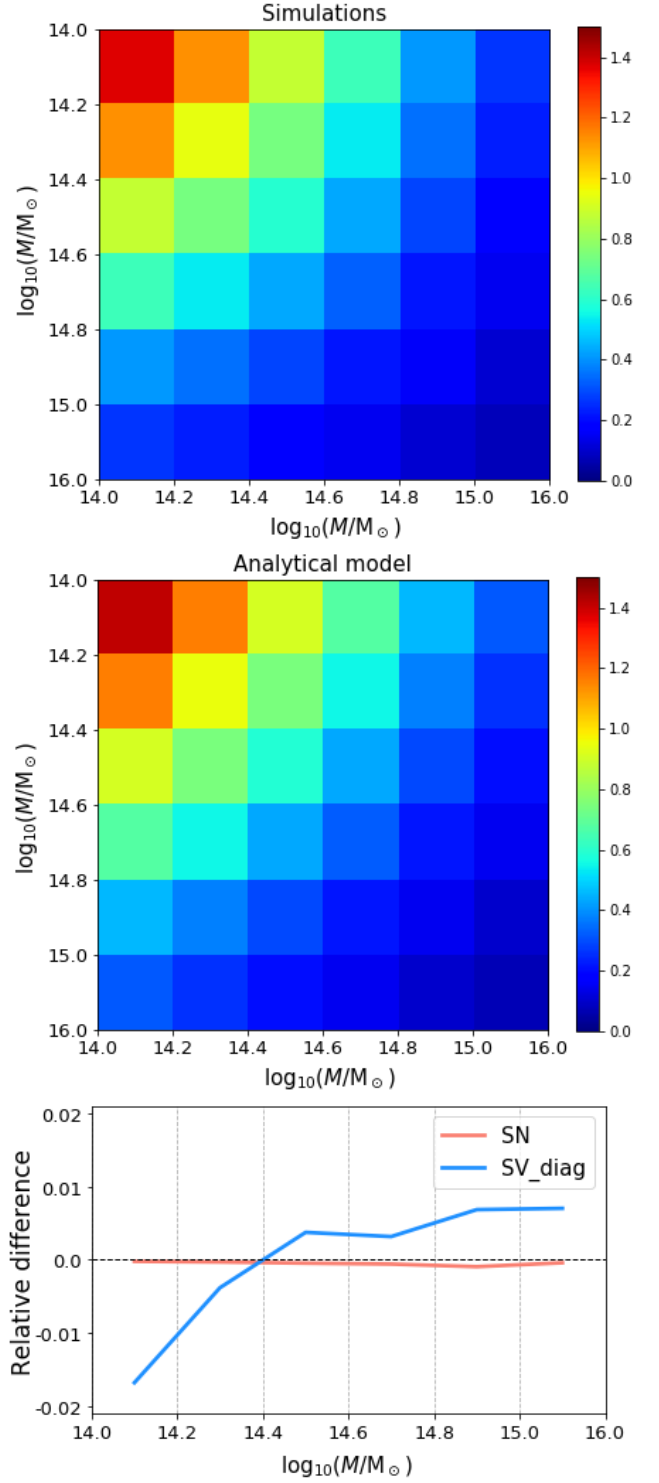
Fig. A.1. Normalized sample covariance between mass bins from simulations ( top ) and our analytical model ( center ), computed for 10^6 spherical sub-boxes of radius R = 200 h^{-1} \text{ Mpc} at redshift z = 0.506 and in the mass range 10^{14} \leq M/M_\odot \leq 10^{16} . In the bottom panel , relative difference between simulations and model for the diagonal elements of the sample covariance matrix (blue) and for the shot-noise (red).
