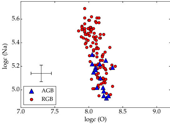
Figure 5. O and Na abundances for our M 4 sample. The error bar indicates typical 1\sigma total uncertainties in individual abundances (i.e. the line-to-line uncertainties and the 1\sigma atmospheric sensitivity uncertainties added in quadrature).
