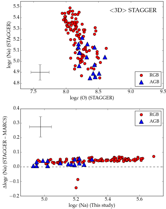
Figure 21. Top panel: Na and O abundances for each star in our M4 sample, determined using the non-LTE BALDER code with the (3D) STAGGER-grid of stellar atmospheric models (see §6.3 for details). Error bars indicate our total abundance uncertainties (Table 7). Bottom panel: The star-to-star differences in Na abundance as determined using the non-LTE BALDER code with i) the 1D MARCS, and ii) the (3D) STAGGER-grid of atmospheric models. The two outlying stars with negative differences are the two brightest stars in our sample, and were outside the STAGGER-grid by \sim 1.0 dex in \log g . Error bars indicate our total uncertainty in Na abundance.
