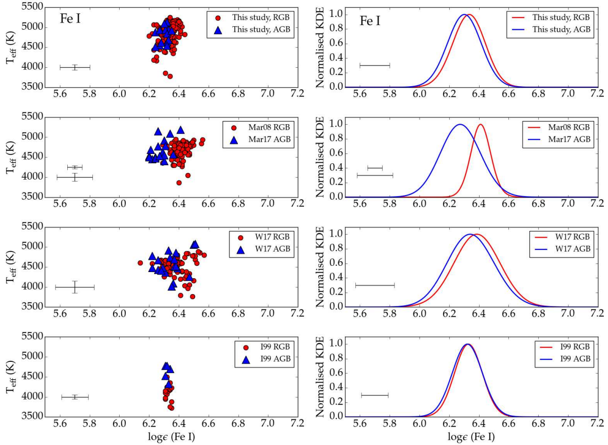
Figure 9. Abundances determined from Fe I absorption lines from this study, Mar17 , Mar08 , W17 , and I99 are presented in the left-hand panels, with kernel density estimations (KDEs) of these data presented in the right-hand panels. Typical abundance errors are shown, as published in the relevant studies (in the Mar17 / Mar08 panel the top error bars are those of the RGB sample in Mar08 ), and were used as the bandwidths of the KDEs in the right-hand panels.
