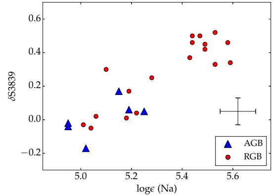
Figure 8. \delta S3839 (excess CN index values) versus Na abundances for stars in both our M4 HERMES and AAOmega samples. \delta S3839 values are the distance a star is above the green trend-line in Figure 7. The error bar represents typical uncertainties. Note that for two stars (25133 and 17999) only low-resolution spectra were observed, and they are therefore not included in this plot.
