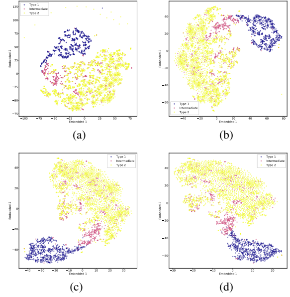
Fig. A.5. t-SNE for whole dataset scaled and mean normalized with various perplexity values. Color-coding of points as in Fig. 4. (a) Perplexity: 5 (b) Perplexity: 15 (c) Perplexity: 30 (d) Perplexity: 40.
