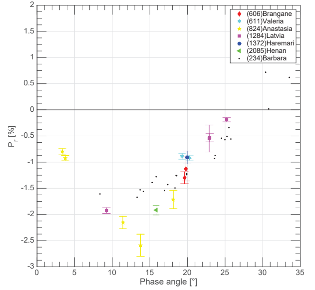
Figure 9: Polarimetric data for (606) Brangane (red diamonds), (824) Anastasia (yellow pentagrams), (1284) Latvia (magenta squares), (1372) Haremar (large blue disk), and (2085) Henan (green triangle). Polarimetric data of (234) Barbara are also shown as small black points for a comparison.
