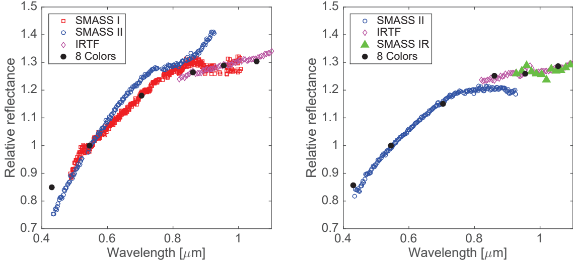
Figure 2: Example of Visible-Near-infrared merging issues for (234) Barbara (left part) and (236) Honoria (right part). SMASS I data are represented by red squares, SMASS II by blue circles, SMASS IR by green triangles, IRTF by purple diamonds, and ECAS data by black dots.
