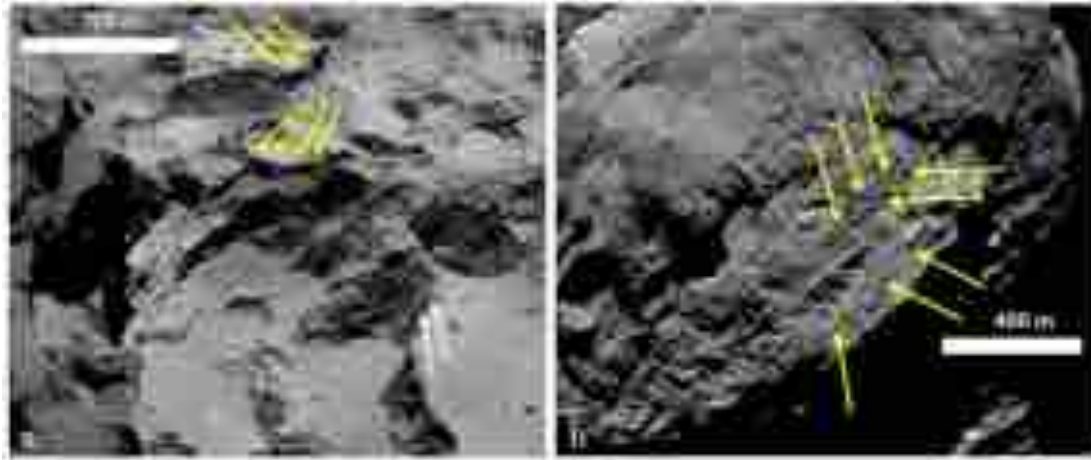
Figure 3. Examples of the linear features. (a) White arrows point out the strata on the cliff, whereas the topmost layer of the strata sequence corresponds to terrace planes and cuesta gentle slopes (yellow arrows). (b) Yellow arrows indicate long fracture systems on Wosret.
