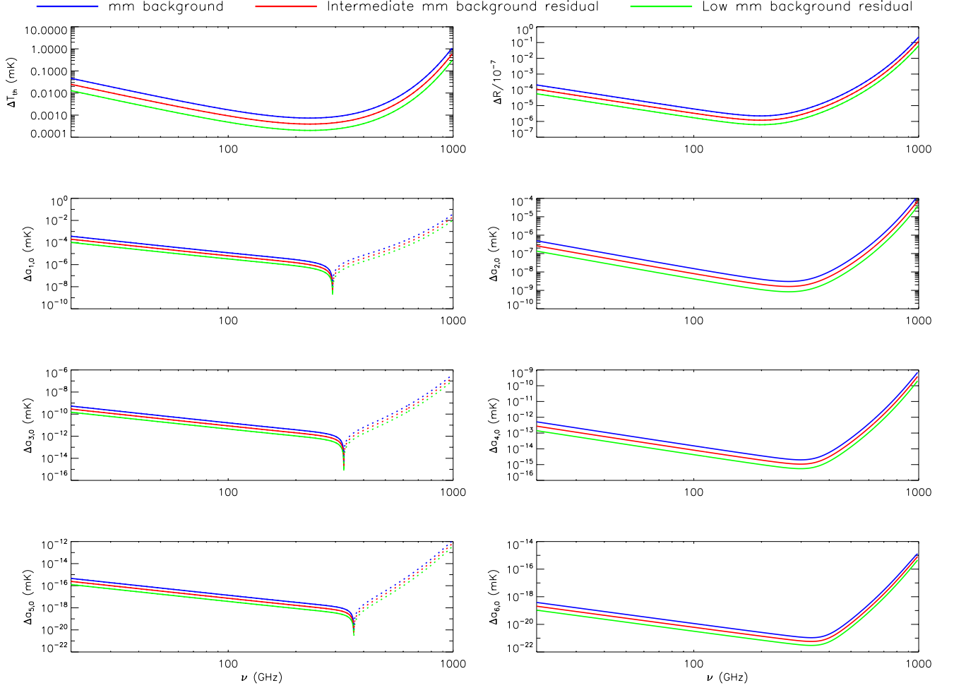
Fig. 6. \Delta T_{th} , \Delta R , and \Delta a_{\ell,0} from \ell = 1 to \ell_{\max} = 6 for the considered millimetre background model from extragalactic radio sources and estimates of extragalactic source millimetre background signal for two assumptions of source contribution subtraction (summed in intensity with the CMB blackbody). Solid lines (or dots) correspond to positive (or negative) values. See also the legend and the text.
