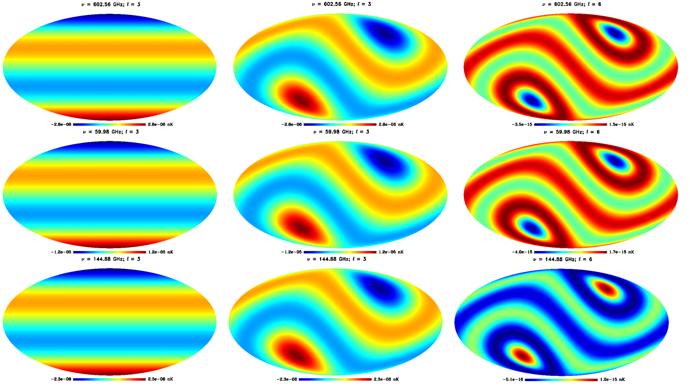
Fig. 10. Examples of maps at two specific multipoles in the reference system with the z axis parallel to the observer velocity (left column) and in Galactic coordinates (central and right columns). According to Planck Collaboration (2020a), we adopt l = 264.021^\circ and b = 48.253^\circ for the dipole direction in Galactic coordinates. We display the temperature pattern for a BE-like distortion with \mu_0 = 1.4 \times 10^{-5} (top row), a Comptonization distortion with u = 2 \times 10^{-6} (central row) and the CIB distribution function with best-fit amplitude value I_0 = 1.3 \times 10^{-5} added to the blackbody one (bottom row), minus the temperature pattern coming from the blackbody. The considered frequency and multipole is given above each map. Maps are in equivalent thermodynamic (or CMB) temperature.
