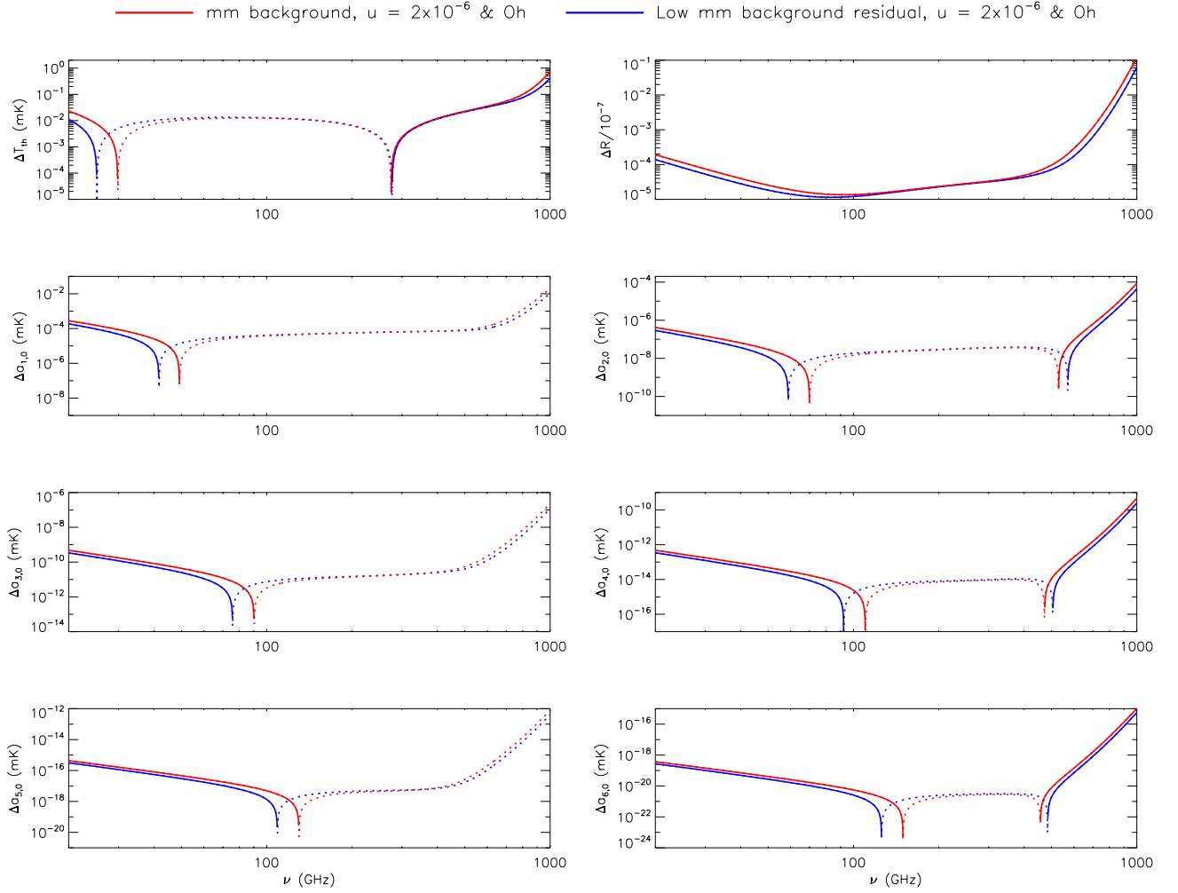
Fig. 8. \Delta T_{th} , \Delta R , and \Delta a_{\ell,0} from \ell = 1 to \ell_{\max} = 6 for the sum of the considered millimetre background model from extragalactic radio sources or an estimate of its residual signal for an assumption of source detection threshold plus a combined Comptonization and diffuse FF distortion model. Solid lines (or dots) correspond to positive (or negative) values. See also the legend and the text.
