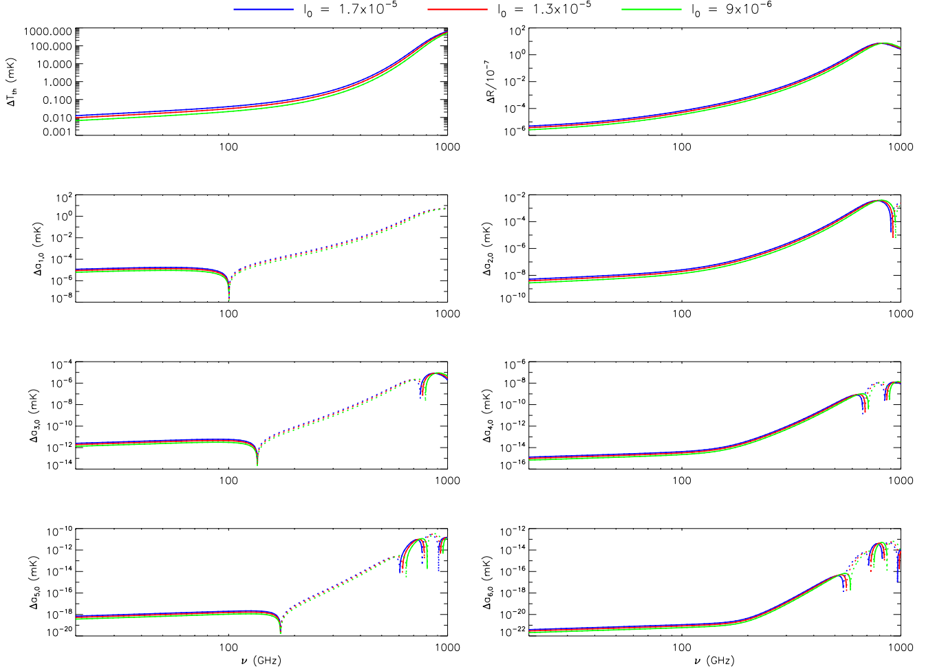
Fig. 7. \Delta T_{th} , \Delta R , and \Delta a_{\ell,0} from \ell = 1 to \ell_{\max} = 6 for the considered CIB models (summed in intensity with the CMB blackbody). Solid lines (or dots) correspond to positive (or negative) values. See also the legend and the text.
