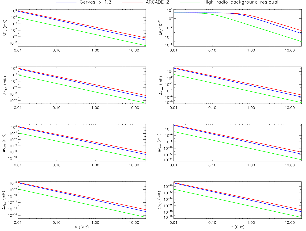
Fig. 5. \Delta T_{th} , \Delta R , and \Delta \alpha_{\ell,0} from \ell = 1 to \ell_{\max} = 6 for the two considered extragalactic radio background models and an estimate of extragalactic radio source background signal for an assumption of source contribution subtraction (summed in intensity with the CMB blackbody). Solid lines (or dots) correspond to positive (or negative) values. See also the legend and the text.
