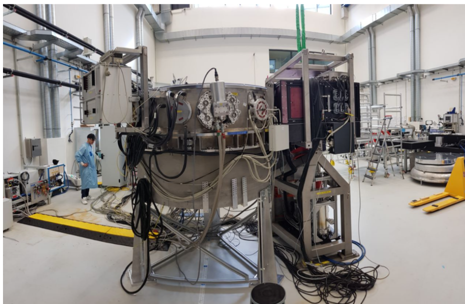
Figure 1. CRIRES + integrated in the laboratory at ESO Garching, Germany. On the right the warm optical bench is enclosed in a black cover. The cryogenic dewar is on the left side of the picture.
