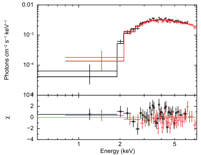
Figure 2. Merged \pm 1 st order MEG (black, box symbol in the residuals) and HEG (red) spectra with best-fit \text{tbabs}*\text{po} model. See Table 2 and Section 3.1.1.
