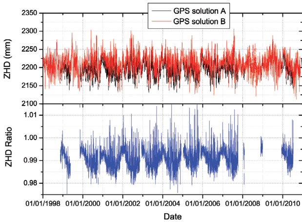
Figure 4. Top: Solution A (black), the ZHD time series for TNB1 obtained by interpolating the grid model values provided with the VMF1 mapping function coefficients ( http://ggsatm.hg.tuwien.ac.at/DELAY/ ). Solution B (red), the ZHD time series obtained with Equation (6) and the surface pressure p data recorded at MZS by the automatic weather station Eneide. Bottom: Ratio of the ZHD times series (Solution A/Solution B; blue) shown in the top plot. The bias between the two series is represented by the discrepancy from unity. The seasonal variations of the bias are also evident.
