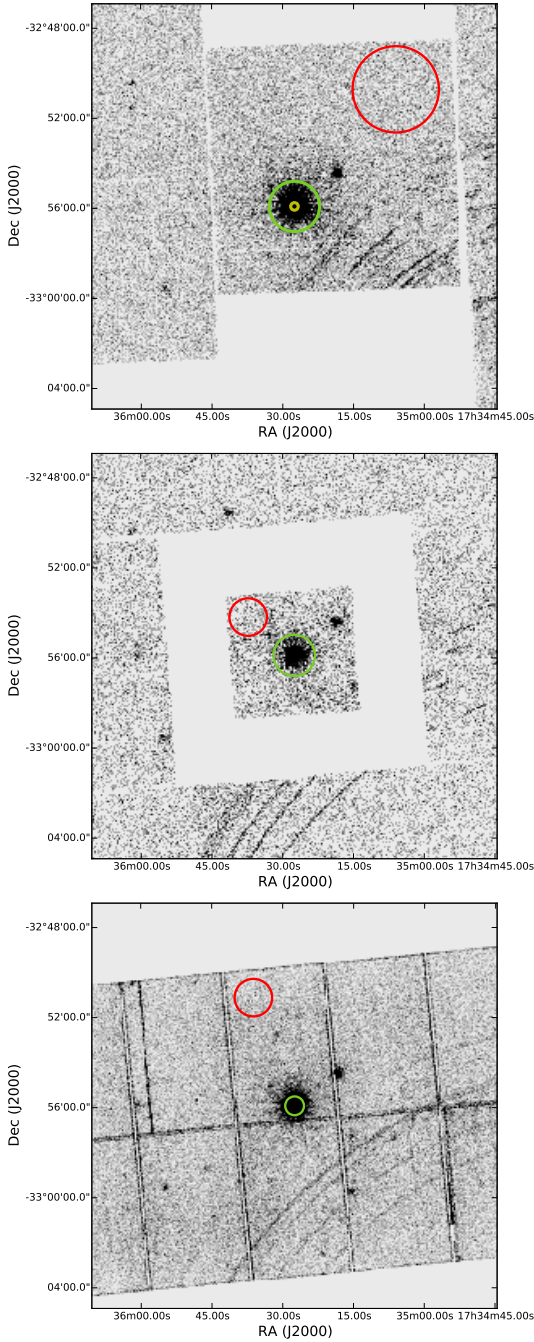
Figure 2. EPIC-MOS1, EPIC-MOS2 and EPIC-pn images for observations one, two and three, respectively. The source and background extraction regions are shown as green and red circles, respectively. The excised inner source region in observation one is shown in yellow.
