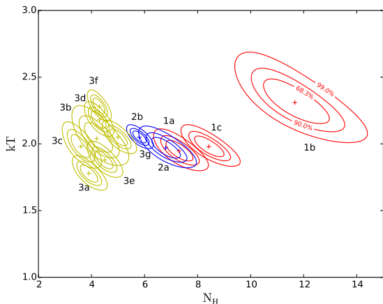
Figure 4. Contour plots for the spectral parameters measured from all observations (Observation one is red, observation 2 is blue and observation 3 is yellow). The contours correspond to the 68%, 90% and 99% confidence levels.
