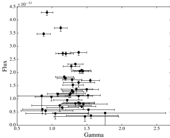
Figure 5. Time-resolved analysis of flux and photon index through observations two and three. Each data point is derived from a 1000s subsection of data.
