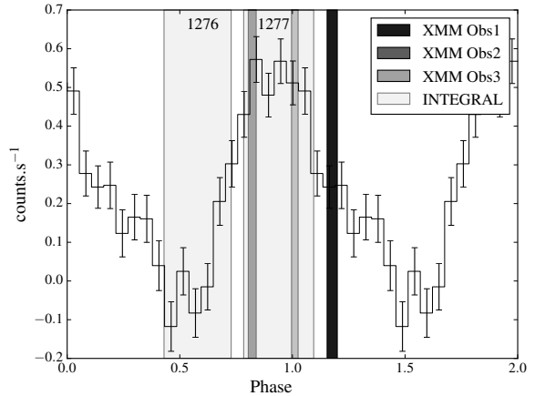
Figure 1. Phase folded light curve of the IBIS/ISGRI data set for IGR J17354–3255 in the 18–60 keV energy band with the ephemeris MJD 55925.895 as phase=0 and a period of 8.447 days. The durations of the three XMM-Newton observations as well as the 327 ks on-source INTEGRAL coverage are indicated according to phase. The two INTEGRAL revolutions are marked by their respective numbers.
