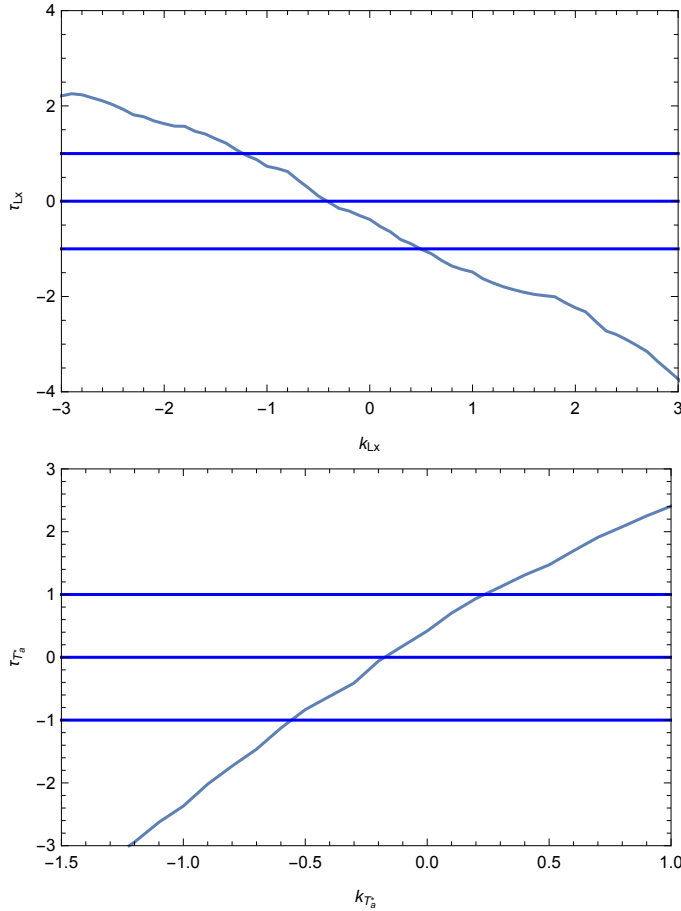
Fig. A.2. Upper panel: test statistic \tau vs. k_{Lx} , the luminosity evolution defined by Eq. (A.1) using a simple power law as g(z) . Lower panel: test statistic \tau vs. k_{T_s} , the time evolution defined by Eq. (A.1).
