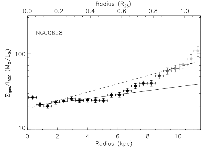
Figure 8. Radial variation of the ratio of gas-mass surface density to SPIRE 500 surface brightness, \Sigma_{\text{gas}}/I_{500} for the face on spiral NGC 628. At \sim 0.7 R_{25} , a change in how the ratio varies with radius is visible. The grayscale shading of the data indicate the fraction of significant pixels with signal to noise greater than three. Overplotted are two lines showing the inverse of the metallicity gradient determined by Moustakas et al. (2010) using the Pilyugin & Thuan (2005) (solid line) and Kobulnicky & Kewley (2004) (dashed line) calibrations. Both lines have been normalized to the value of \Sigma_{\text{gas}}/I_{500} at 0.1 R_{25} . (The complete figure set (28 images) is available.)
