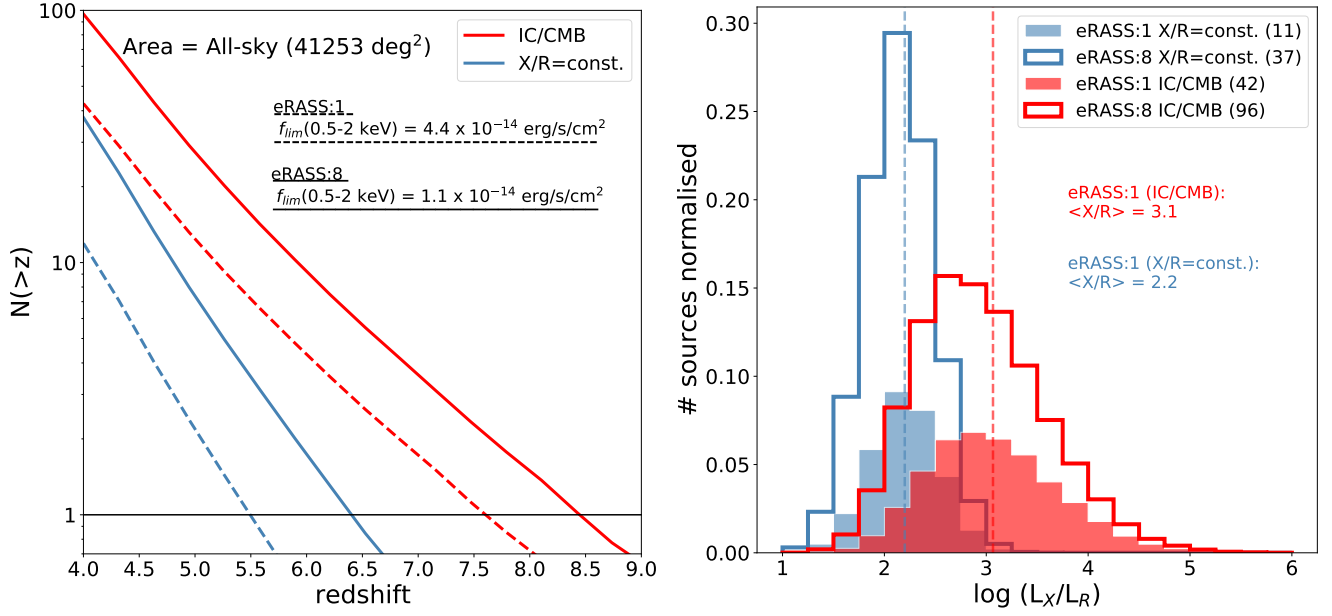
Figure 5. Prediction of the number (left panel) and properties (right panel) of z > 4 blazars expected to be found with the eROSITA all-sky survey. In both panels red lines represent the estimates made considering the IC/CMB model, whereas blue lines indicate the estimates assuming non-evolving X/R ratios. Dashed lines and filled histograms refer to the predictions after the first scan of the sky (eRASS:1), while the continuous lines and empty histograms are for 8 scans (eRASS:8). Left: Expected number of detected blazars above a given redshift as a function of redshift. Right: X-ray-to-radio ratio distributions. The dashed vertical lines indicate the mean values expected in the eRASS:1. Both filled and empty histograms have been normalised dividing by the total number of blazars expected in the eRASS:8 considering the corresponding evolving scenario. In the legend, the total number of blazars expected to be observed for each scenario is reported in brackets.
