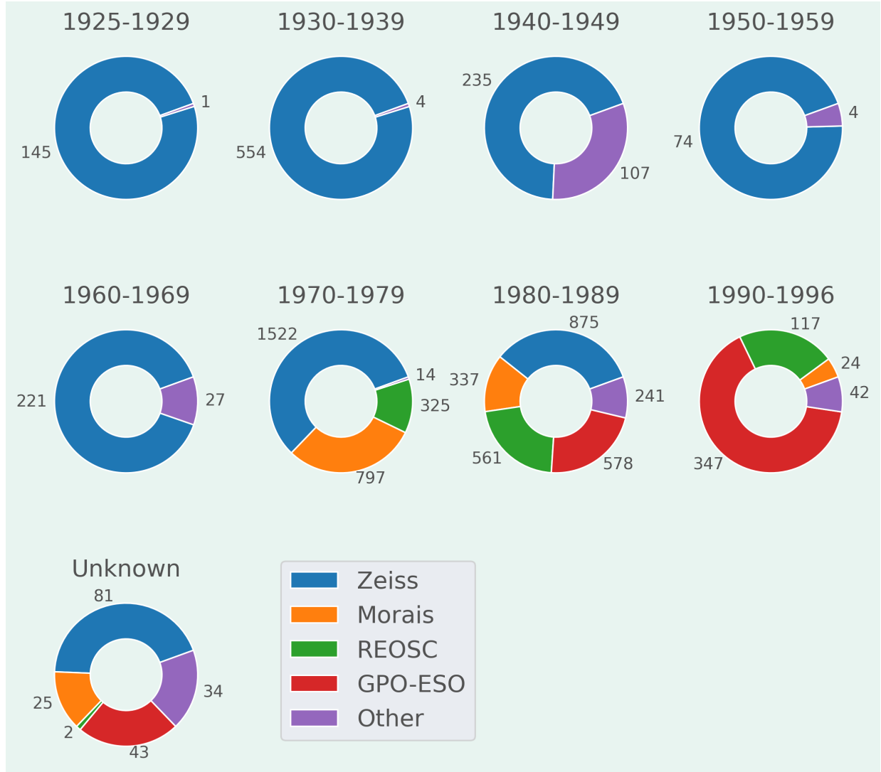
Figure 6: Pie charts showing which telescopes have been used in different ranges of epoch and the correspondent number of plates. The label Other groups all the non-OATo telescopes except ESO-GPO. The bottom-left pie-chart groups plates of unknown epoch.
