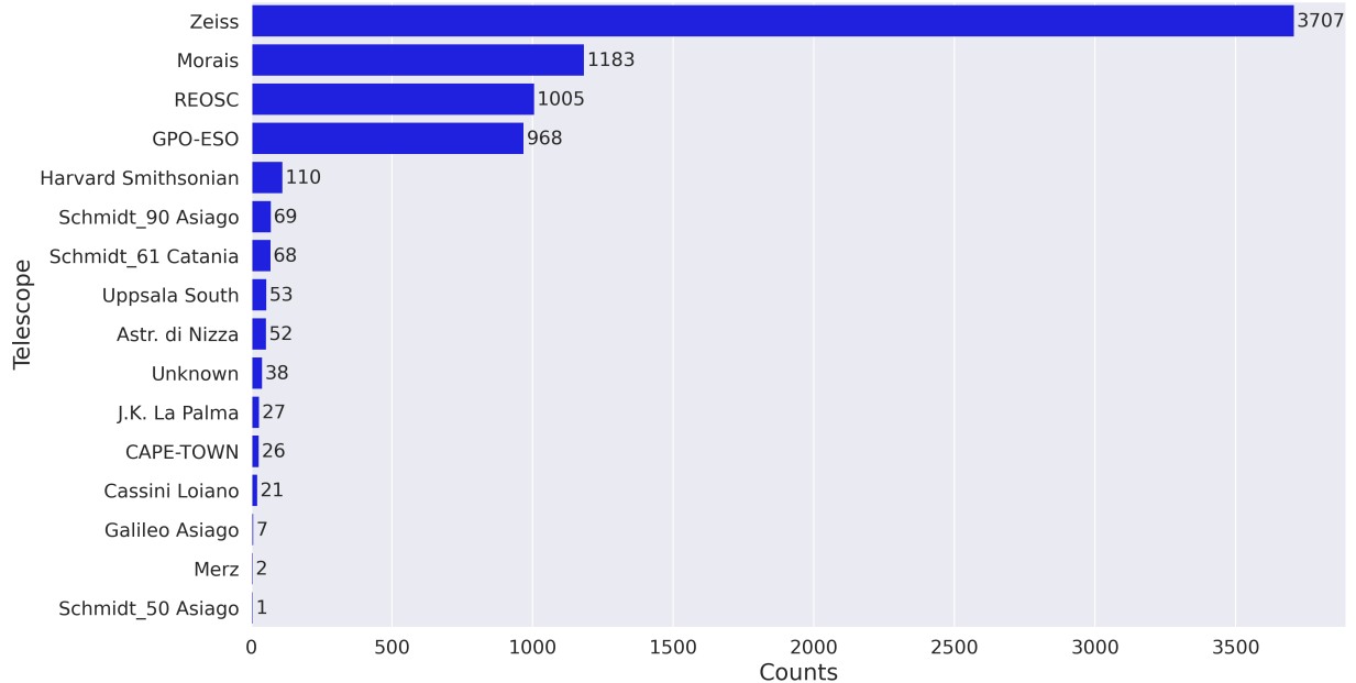
Figure 5: Histogram of the number of plates per telescope.
