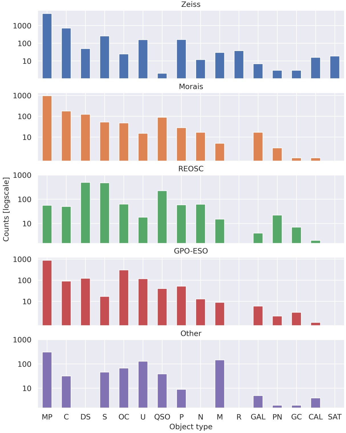
Figure 7: Histograms of the type of objects observed by the main four telescopes (top 4 panels). The bottom panel groups others non-OATo telescopes ( Other ).
