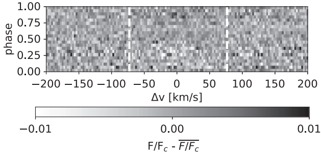
Figure 4. Evolution of the LSD residuals with respect to the time averaged profile from HERMES. The phase of the star is normalized to the rotation period, assuming the 0.88 d value. The vertical dashed lines represent the \pm v \sin i values to delimit the width of the spectral line.
