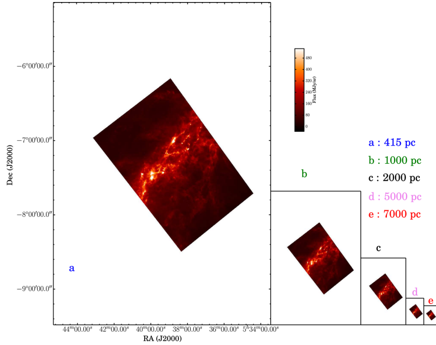
Figure A8. Original and moved Orion A centre maps at 250 \mu\text{m} .
