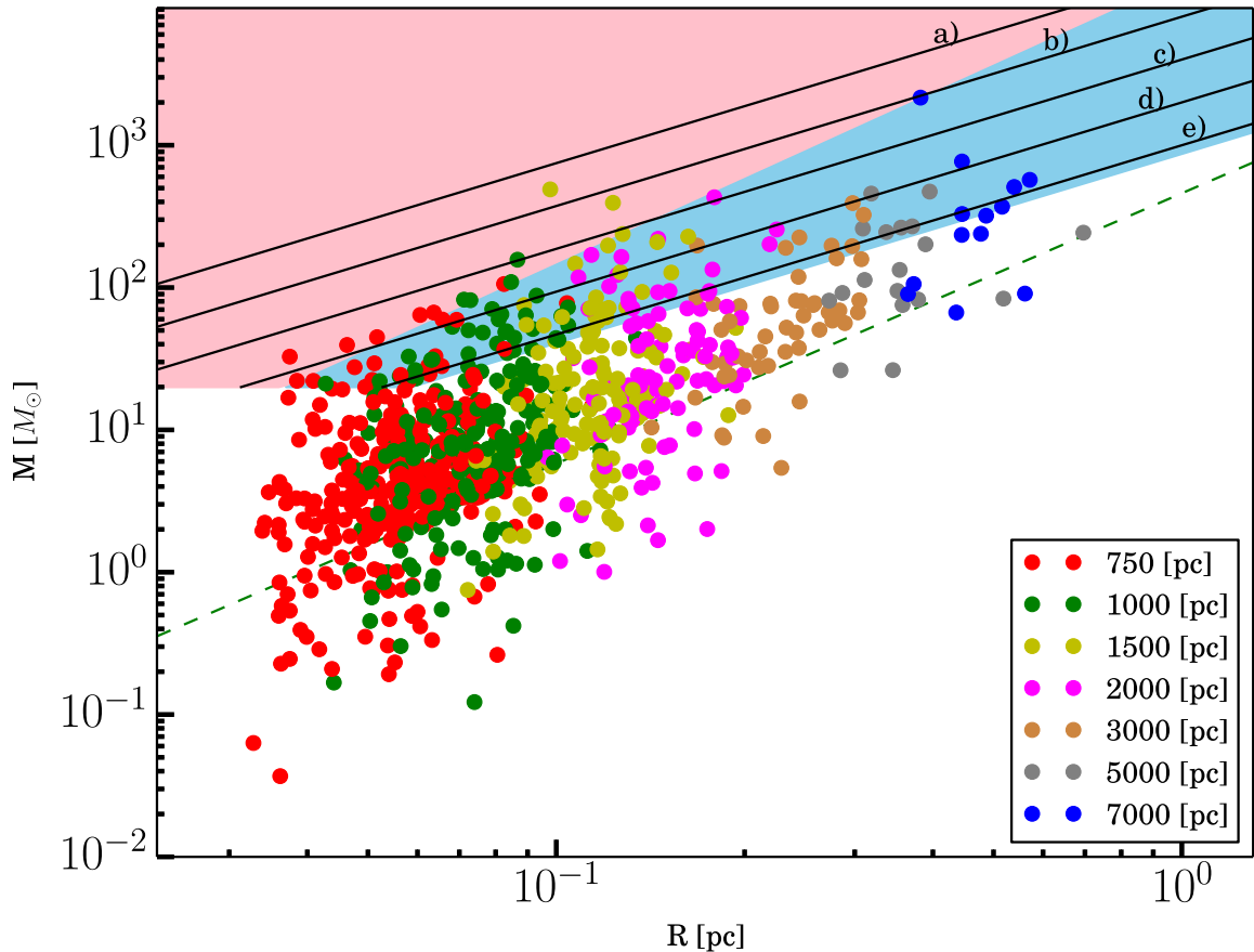
Figure 29. MR plot containing all the sources (solid circles) detected at each virtual distance being associated with sources detected in the original map that are below the MSF zone (FP and TN). Black solid lines are lines parallel to the KP relation M = k r^{1.33} . The (a) line is for k = 16000 and delimits the probability of getting an FP above this line, (b) is for k = 8000 , (c) to k = 4000 , (d) to k = 2000 and (e) k = 1000 . The k = 870 line coincides with the KP relation. The probability values p(k) (equation 8) are shown in Table 2. Dashed green line is the so-called Larson's third law (see equation 5). Pink and sky-blue zones correspond to thresholds of KM and KP, respectively.
