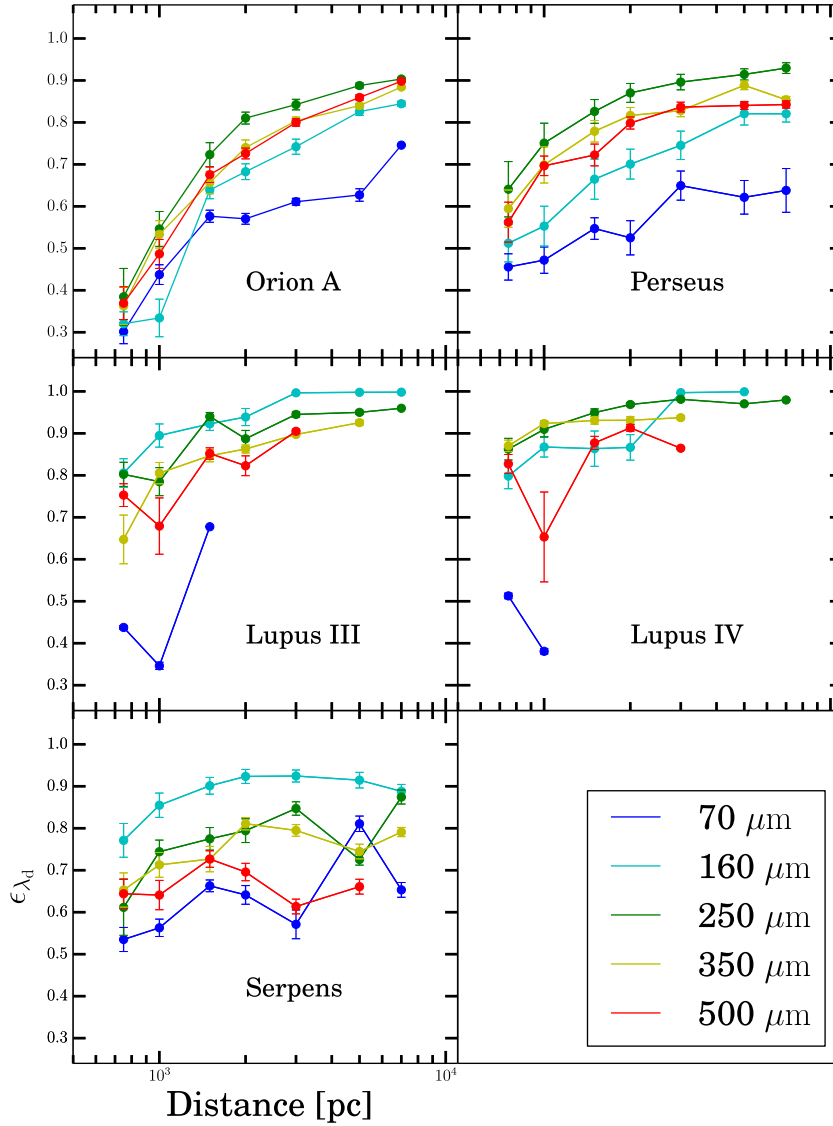
Figure 10. Mean fraction of diffuse emission \epsilon_{\lambda(d)} = \langle (F_{\lambda(d)} - F_{\lambda_{\text{ad}}}) / F_{\lambda(d)} \rangle versus virtual distance.
