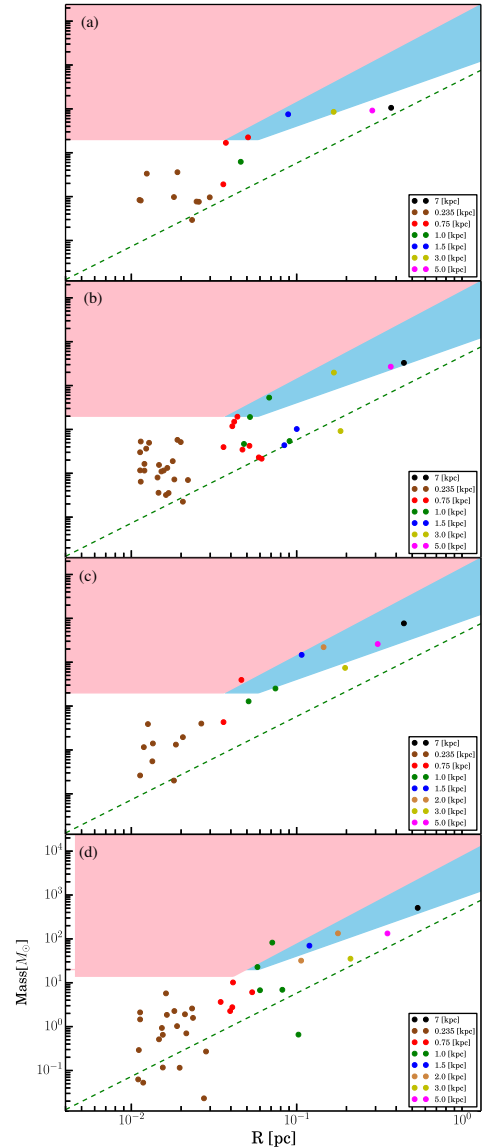
Figure 23. MR plots of sources found in the Perseus maps moved to various distances. Each plot is built starting from one of the four sources found at the largest distance (7 kpc), and contains all the sources found at shorter distances and contained in it.
