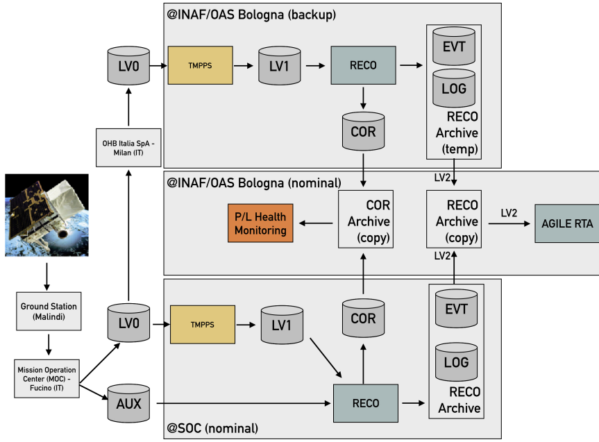
Fig. 1 The data flow from LV0 to LV3 for the second version of the AGILE Real-Time Analysis. TMPPS and RECO runs at SOC in SSDC and produce a COR and a RECO Archive that are transferred to INAF/OAS Bologna. A backup chain from Telespazio to OHB Italia SpA (formerly Compagnia Generale dello Spazio (CGS)), Milan is also present. The P/L Health monitoring is used by MOC people to check the status of the P/L.
