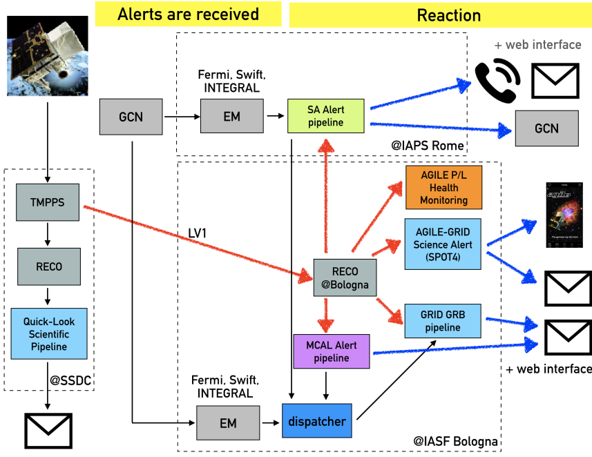
Fig. 5 The first version of the AGILE Real-Time Analysis workflow at INAF/OAS Bologna (formerly INAF/IASF), INAF/IAPS Rome and SSDC, in operation until 2016, with the LV1 data received from SSDC. Alerts are received from the GCN network. The AGILE-GRID Science Alert System (SPOT4) the AGILE-MCAL and SA Alert pipelines analyze new data as soon as is processed by RECO-STD, that perform the reconstruction of the data. The AGILE-GRID GRB pipeline reacts if there are GRBs notified by the GCN network or detected by SA and MCAL pipelines (via the dispatcher). A web GUI and the AGILEScience App show the results of some automated processing. Alerts are sent by email to the AGILE Team. The SA Alert pipelines run at INAF/IAPS Rome and has a wake-up system and was able to generate GCN notices.
