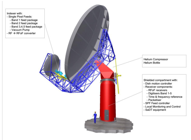
Figure 1: SKA DISH overview.
