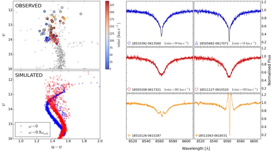
Figure 2. Left-upper panel: observed v –( u - v ) CMD of M11. Spectroscopically analyzed stars are marked with large circles. The color of each circle is associated with the corresponding value of v \sin i as indicated by the color scale on the right. Left-lower panel: v –( u - v ) synthetic CMD corresponding to two coeval populations (age = 250 Myr), one with no rotation (blue) and the other with high rotation ( \omega = 0.9\omega_{\text{crit}} , red). The expected photometric error has been added to the simulations. Right panels: some examples of our spectra. From the upper to lower panels we show two bMS and two rMS at similar magnitude, and two \text{H}\alpha core emission stars. For each bMS and rMS spectrum, we superimpose to the observed spectra the best-fitting non-LTE model in black.
