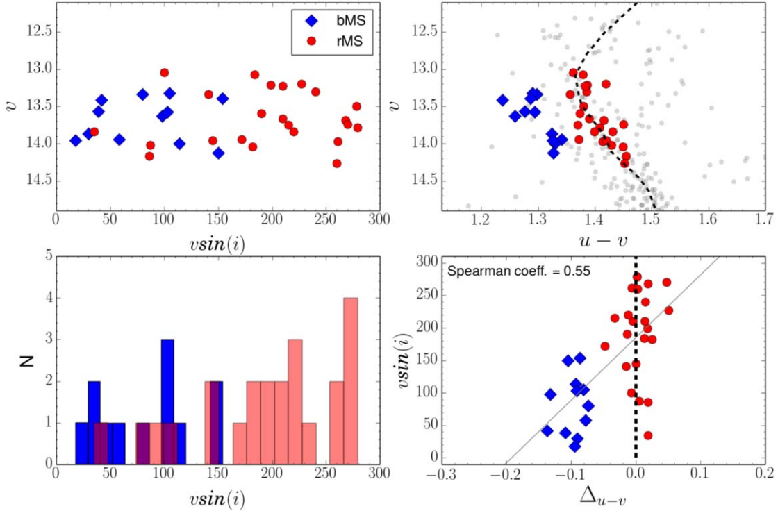
Figure 3. Left: v mag vs. v \sin i for MS stars in M11 (upper panel); on the lower panel we show the histogram distribution of v \sin i for rMS (red) and bMS (blue). Right: v –( u - v ) CMD zoomed on the MS. The black-dashed line is a fiducial for the rMS (upper panel). The lower panel shows v \sin i as a function of the difference between the (u - v) color of each MS star and the color of the fiducial ( \Delta_{u-v} ). The black-dashed line corresponds to \Delta_{u-v} = 0 . In all panels rMS and bMS are represented with red-filled circles and blue diamonds, respectively.
