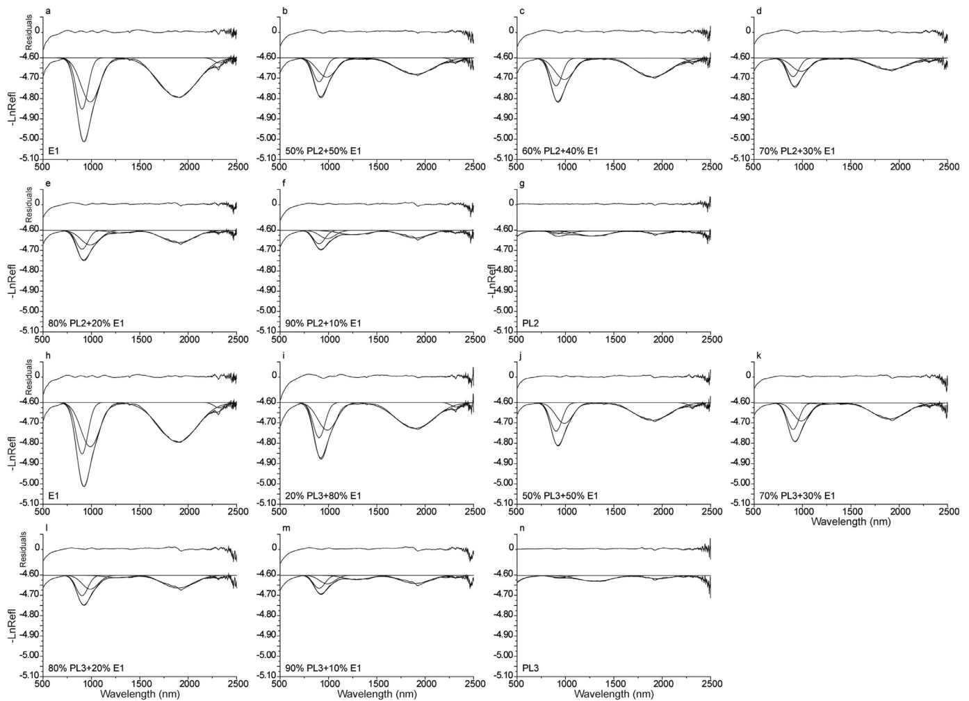
Fig. 5. MGM deconvolution and residuals of E1-bearing mixtures. RMS values are consistent with Klima et al. (2011). (a–g) E1–PL2 mixtures; (h–n) E1–PL3 mixtures. Continuum-removed reflectance is expressed as -\text{LnRefl} .
