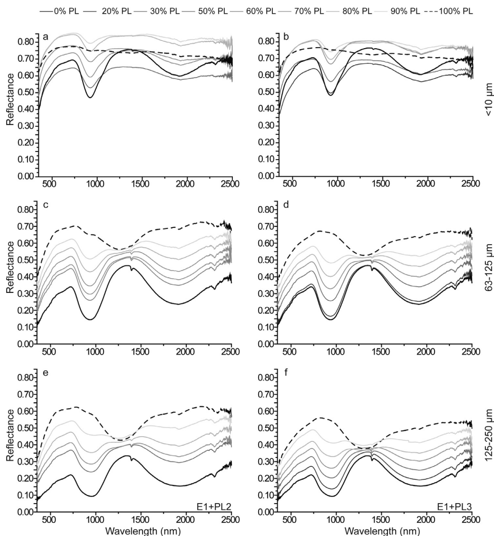
Fig. 2. Reflectance spectra of E1-PL mixtures at three different particle sizes. (a, b) E1+PL2 and E1+PL3, <10\mu\text{m} ; (c, d) E1+PL2 and E1+PL3, 63\text{--}125\mu\text{m} ; and (e, f) E1+PL2 and E1+PL3, 125\text{--}250\mu\text{m} . Generally, a fine particle size produces spectra with higher reflectance and reduced spectral contrast compared to the coarsest sizes.
