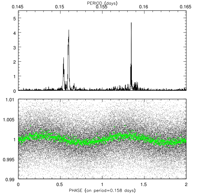
Fig. 5. Top panel: periodogram of the 20 quiescent intervals of Fig. 3, searched together. Bottom panel: light curve data points from the 20 intervals phased on the period 0.15845058 d ( \sim 3.8 h, black points). The green crosses represent a phase binned version of the same light curve (bin size 50 data points).
