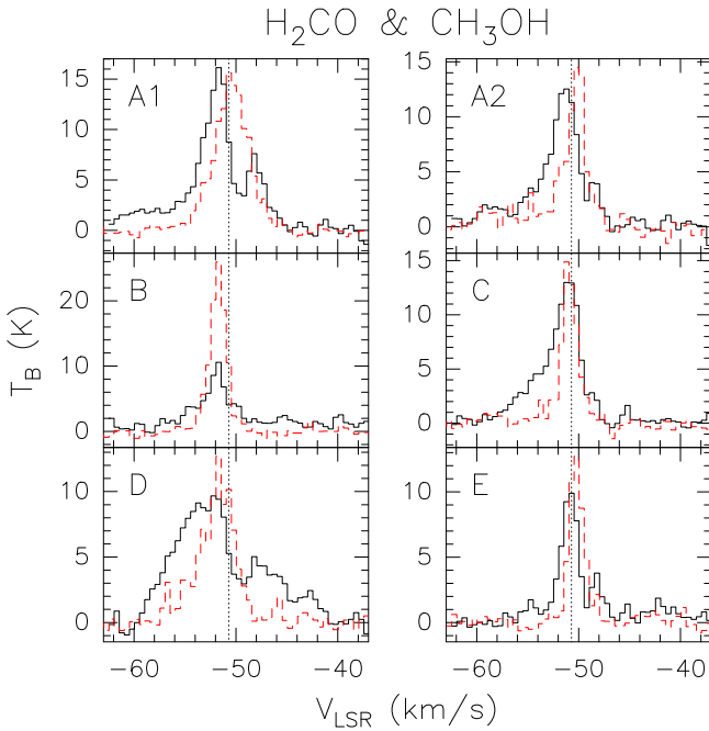
Fig. 14. Spectra of the \text{H}_2\text{CO}(3_{03}-2_{02}) (black solid histogram) and \text{CH}_3\text{OH}(4_2-3_1) E1 (red dashed histogram) lines towards the positions of the six cores identified in IRAS 23385+6053. The vertical dotted line is shown to ease the comparison between spectra of different cores.
