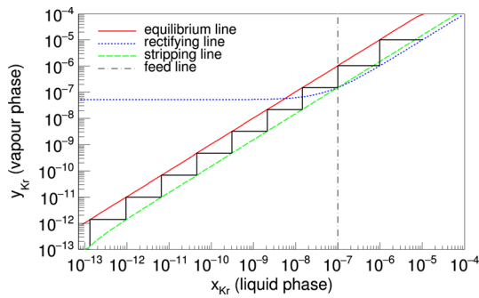
Fig. 2 McCabe–Thiele diagram for the XENON1T requirements. The concentration of the krypton in the gas phase y_{Kr} in relation to the concentration in the liquid phase x_{Kr} . The operation lines for the different sections, namely rectifying (blue dotted line), stripping (green dashed line) and feed line (grey dash-dotted line) of the column are drawn and allow for the determination of the number of theoretical stages needed to meet the XENON1T requirements (black solid line). The definitions of the equilibrium (red solid line) and operation lines are taken from [12, 14]
