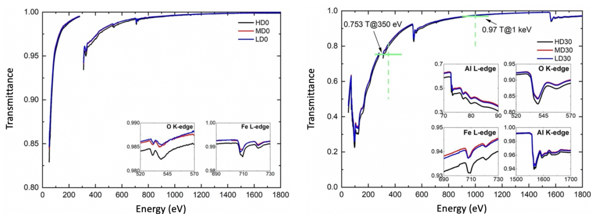
Figure 4. Comparison of HD/MD/LD with no Al (left) and with 30 nm of Al (right). The transmittance requirements at 350 eV and at 1 keV are reported in green.
