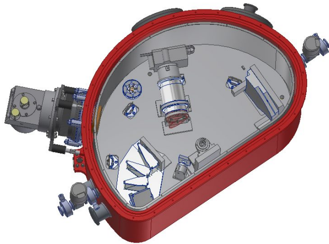
Figure 10. NIR optomechanics.
