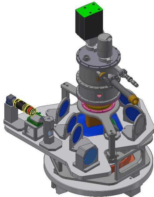
Figure 6. The UV-VIS optomechanics.
