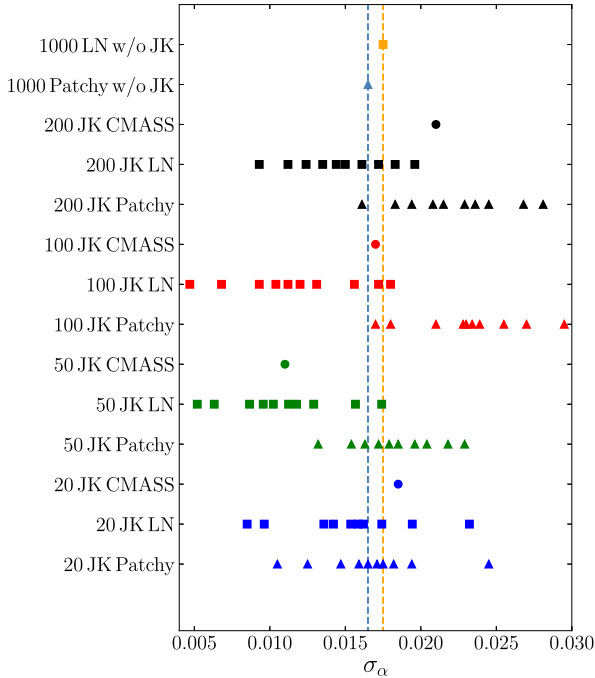
Figure 7. Uncertainties on the \alpha shift parameter obtained from the 1000 Patchy and LN mocks without jackknife, and from the CMASS, 10 Patchy and 10 LN jackknife resamplings. The different sets of points are colour-coded as in Fig. 6 and the vertical lines help the comparison with the ideal cases of 1000 Patchy and LN mocks.
