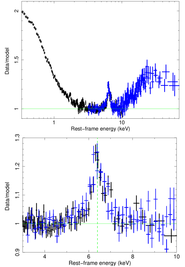
Fig. 2. Data-to-model ratio of the simultaneous 2022 XMM-Newton -pn (black) and NuSTAR (blue) spectrum of ESO 141-G55 fit with a Galactic ( N_H(\text{Gal}) = 5.7 \times 10^{20} \text{ cm}^{-2} ) absorbed power-law continuum model over the 3–5 keV energy range. Top panel: Extrapolation over the 0.3–79 keV broadband X-ray energy range. Bottom panel: Zoom-in on the Fe K\alpha line. The vertical dashed green line corresponds to 6.4 keV.
