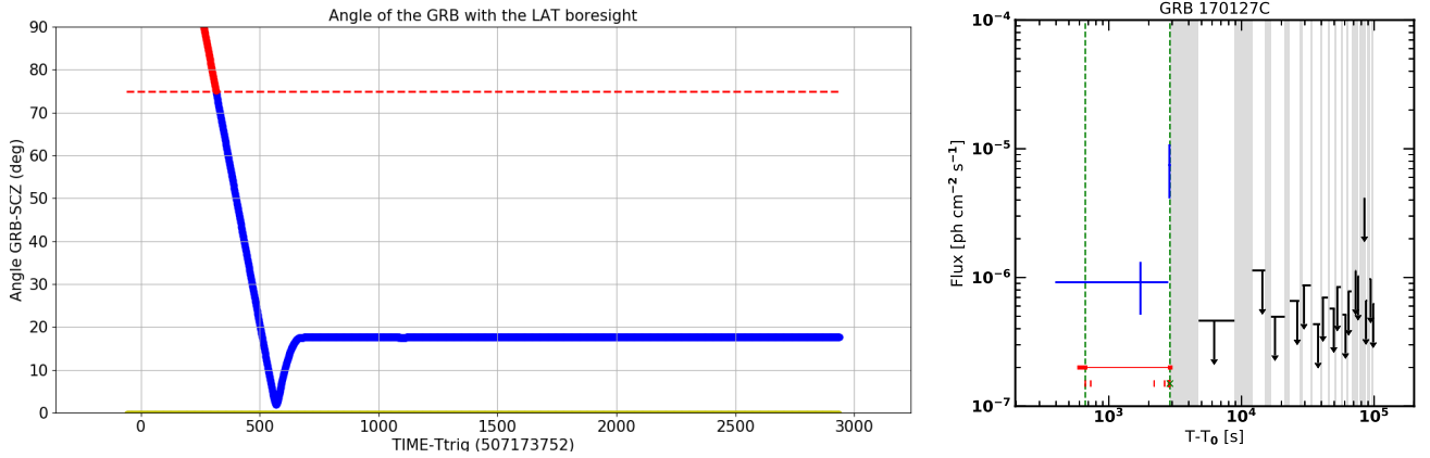
Figure 11. Left panel: Off axis angle for GRB 170127C as a function of time since the GBM trigger. The horizontal red line corresponds at \theta = 75^\circ . Right panel: Temporal extended emission for GRB 170127C. The blue point is the photon flux measurement with a significance of \text{TS} > 10 , while, for lower value of \text{TS} , upper bounds are displayed as black arrows. The horizontal red line indicates the estimated duration of the burst, and the thick parts of it correspond to the uncertainty on the T_{\text{LAT},0} and T_{\text{LAT},100} parameters. The red vertical markers indicate the arrival time of each photon with probability > 90\% to be associated with the GRB, with the green cross being the event with maximum energy.
