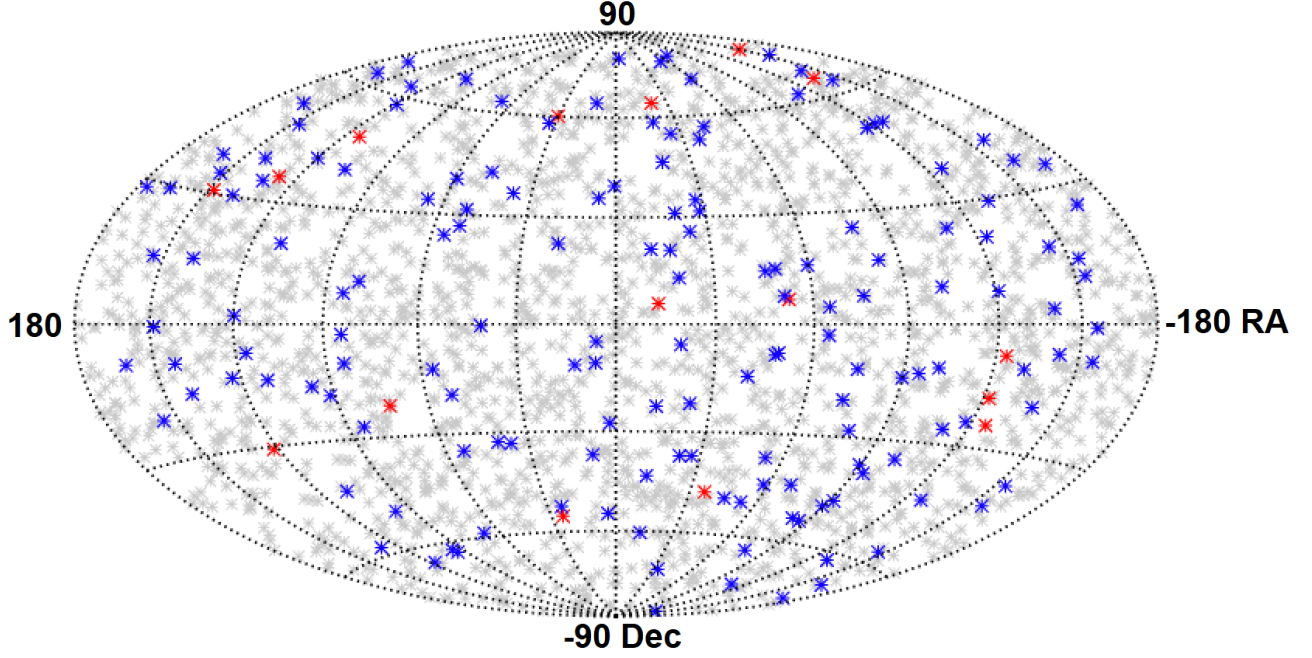
Figure 5. Sky distribution of 2357 GBM-triggered GRBs (from 2008 July 14 to 2018 July 31) in equatorial coordinates ( grey asterisks ). Blue (red) asterisks indicate 160 (16) long (short) LAT-detected GRBs included in the 2FLGC over the same time period.
