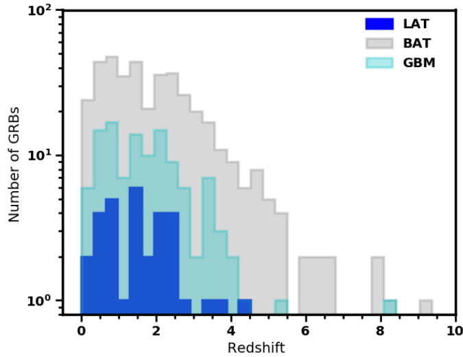
Figure 17. Redshift distribution of 34 GRBs detected by LAT (blue histogram), 405 GRBs detected by Swift -BAT (grey histogram) and 116 GRBs detected by GBM (cyan histogram).
