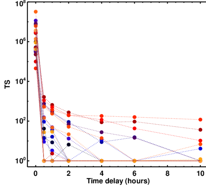
Figure 28. Test Statistic evolution with respect to the time delay (in hours) of the CTA alert reception, obtained from the analysis with a power-law model, with respect to the beginning of the LAT-detected extended emission. The figure shows the TS values for 27 GRBs. For clarity, TS values less than 1 are fixed to 1.
