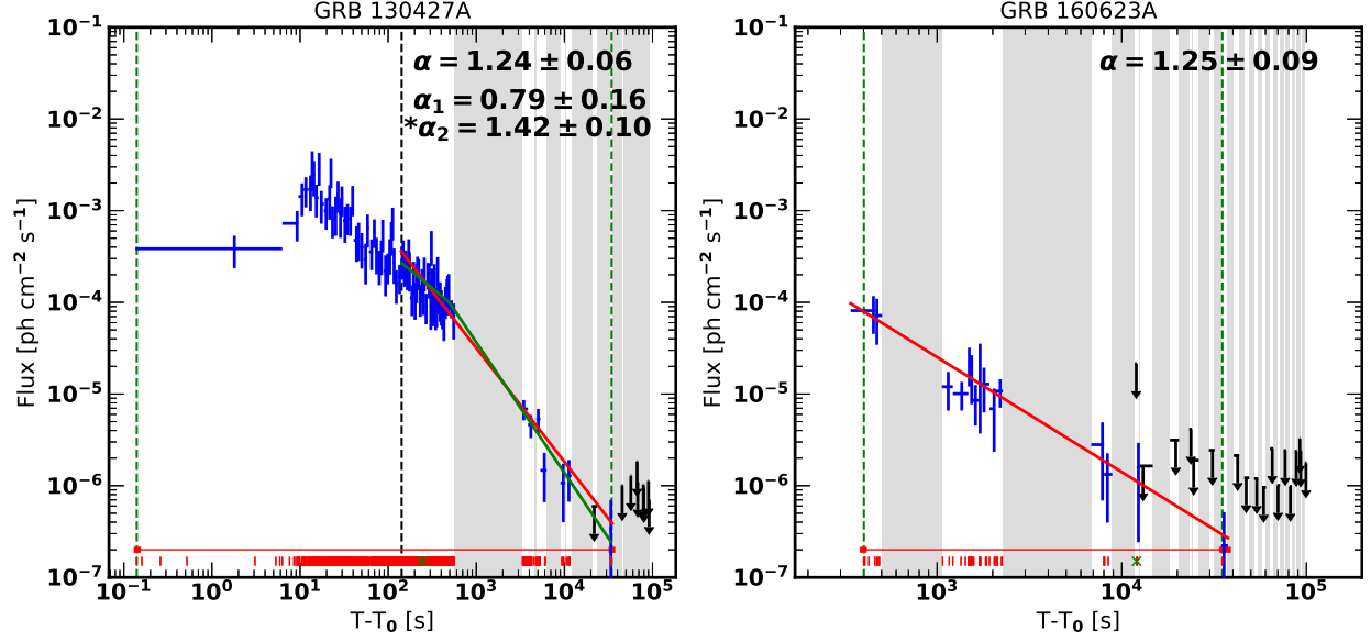
Figure 9. Temporal extended emission for the two longest LAT GRBs, GRB130427A (left panel), and GRB160623A (right panel). For the bright GRB130427A we display the results of the fit for a simple power law model with temporal index \alpha (red line) and with a broken power law with indexes \alpha_1 and \alpha_2 (green line). For GRB160623A, only the result of the fit with a simple power law is shown.
