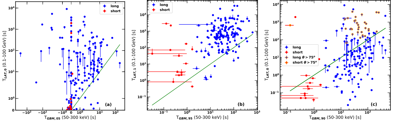
Figure 7. T_{\text{LAT},0} (a) and T_{\text{LAT},1} (b) calculated in the 100 MeV–100 GeV energy range vs. the same quantities calculated in the 50–300 keV energy range. Panel (c) shows the onset times ( T_{\text{LAT},0} ) in the 100 MeV–100 GeV vs. the durations ( T_{\text{GBM},90} ) in the 50–300 keV energy range. The solid line denotes where values are equal. Blue and red circles represent long and short GRBs, respectively. In panel (c), we additionally mark the GRBs which were outside FoV at trigger time with a thick orange contour.
