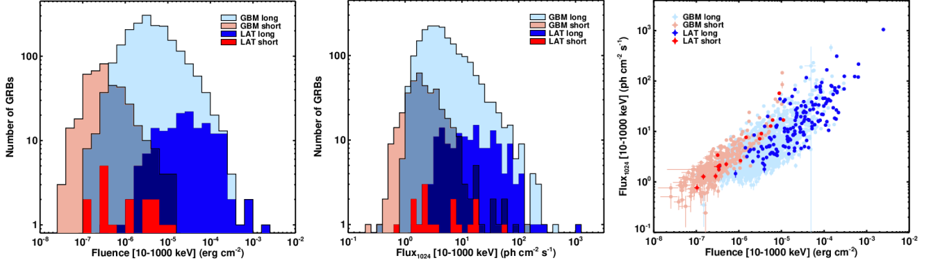
Figure 13. Left panel: The distribution of energy fluence calculated in the 10–1000 keV energy range for 178 bursts detected by the LAT compared to the entire sample of 2357 GRBs detected by GBM over the same time period. Middle panel: The distribution of peak photon flux in the 10–1000 keV energy range for the same sample of LAT and GBM detected populations. Right panel: The GBM peak photon flux (10–1000 keV), as measured on a 1024 ms timescale, versus the energy fluence (10–1000 keV) derived using a spectral model fit to a single spectrum over the entire duration of the burst.
