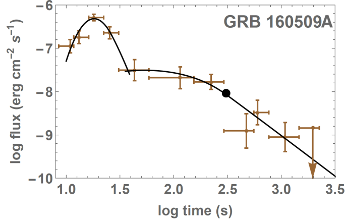
Figure 27. Light curve of GRB 160509A together with the fit using the Willingale et al. (2007) model (solid line). The black dot indicates the end time of the plateau emission and its corresponding flux.
