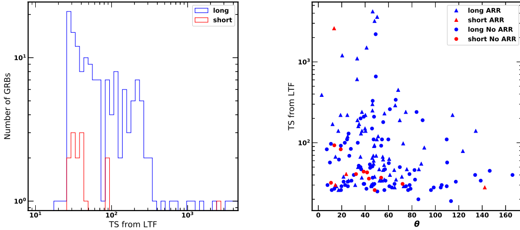
Figure 4. Left panel: Distribution of the Test Statistic (TS) for 14 short (red) and 155 long (blue) GRBs detected by LTF algorithm. Right panel: TS values for long and short bursts as a function of the angle \theta at the trigger time. Bursts which triggered an ARR are marked with a triangle.
