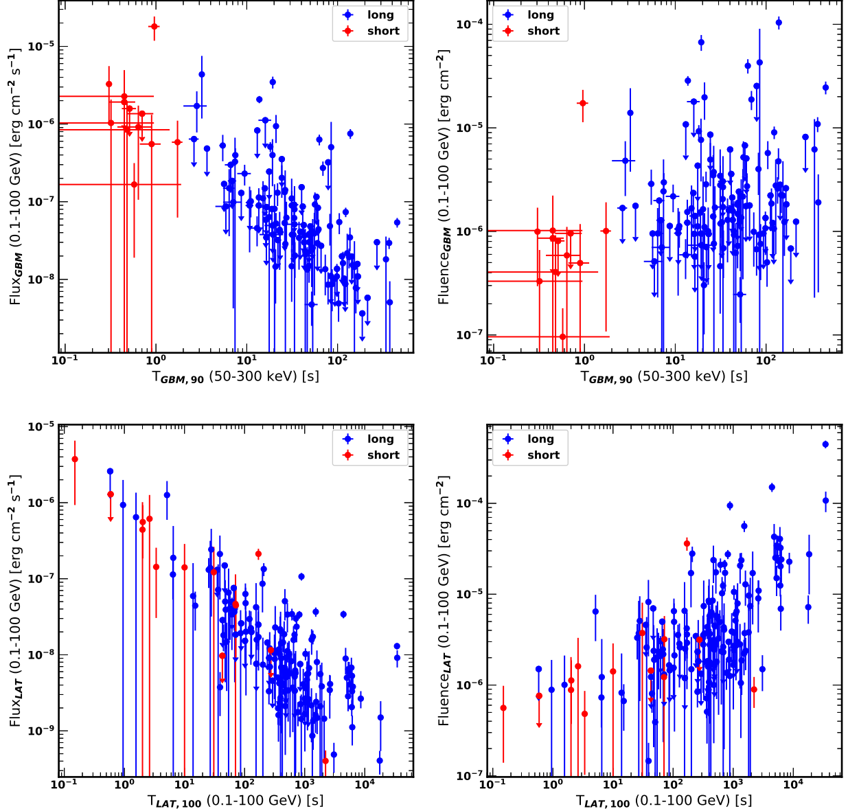
Figure 14. Fluxes (left panels) and fluences (right panels) calculated in the 100 MeV–100 GeV energy range vs. GRB durations. Upper panels show fluxes and fluences evaluated in the “GBM” time window vs. durations calculated in the 50–300 keV energy range ( T_{\text{GBM},90} ). Bottom panels show fluxes and fluences evaluated in the “LAT” time window vs. durations calculated in the 100 MeV–100 GeV energy range ( T_{\text{LAT},100} ). Blue and red circles represent long and short GRBs, respectively.
