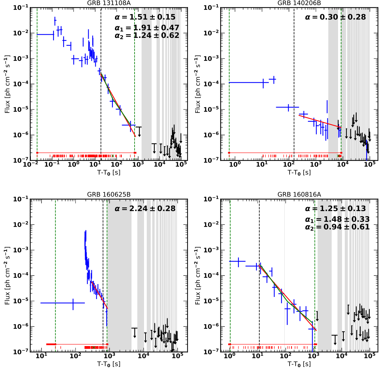
Figure 22. Temporal extended emission for four GRBs showing a peculiar behavior (the name of each GRB is shown in the title of each panel). Markers are the same as Figure 20.
