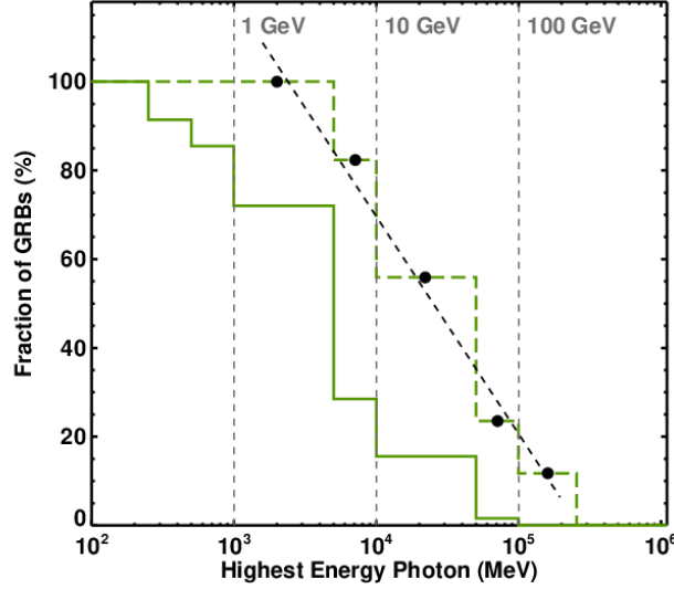
Figure 24. Fraction of GRBs with the highest energy photon detected above selected threshold energies (250 MeV, 500 MeV, 1 GeV, 5 GeV, 10 GeV, 50 GeV) ( green solid line ). The distribution of the source-frame-corrected energies for the redshift sample is indicated with the dashed green line . The dashed black line denotes a linear fit to the values corresponding to the center of each bin.
