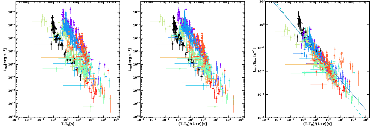
Figure 23. Isotropic luminosity L_{iso} calculated in the 100 MeV–100 GeV rest frame energy range for the 34 GRBs in our sample with measured redshift. The left panel shows L_{iso} vs. the time elapsed since the trigger. GRB 090510 is the only short GRB with known redshift and it is marked with black stars. In the middle panel L_{iso} is plotted against the vs. the time elapsed since the trigger in the rest frame. In the right panel , we show L_{iso} divided by the isotropic energy (calculated in the 1 keV – 10 MeV rest frame energy range) vs. the time elapsed since the trigger in the rest frame. We mark GRB 160623A, which represents an outlier of the distribution (see text for explanation), with orange crosses . The solid line shows a linear fit, giving a decay index of 1.25 \pm 0.03 . For comparison, we also show a dashed line with decay index 10/7 .
