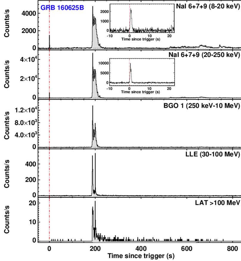
Figure 8. Composite light curve of GRB 160625B: summed GBM/NaI detectors (first two panels), GBM/BGO (third panel), LLE (fourth panel), and LAT rates above 100 MeV (bottom panel). The grey shaded area indicates the T_{\text{GBM},90} calculated in the 50–300 keV energy range. The dashed red lines marks the GBM trigger time. A zoom around trigger time is shown in two insets for each energy range of the NaI detectors, highlighting the peak detected at low energies which caused the trigger in GBM. This peak does not show any counterpart at higher energies. The association of the low-energy ( < 250 keV) late-time emission (from 500 to 800 s post trigger) with the main GRB emission episode has been cross-checked by the GBM Team (FGGC).
