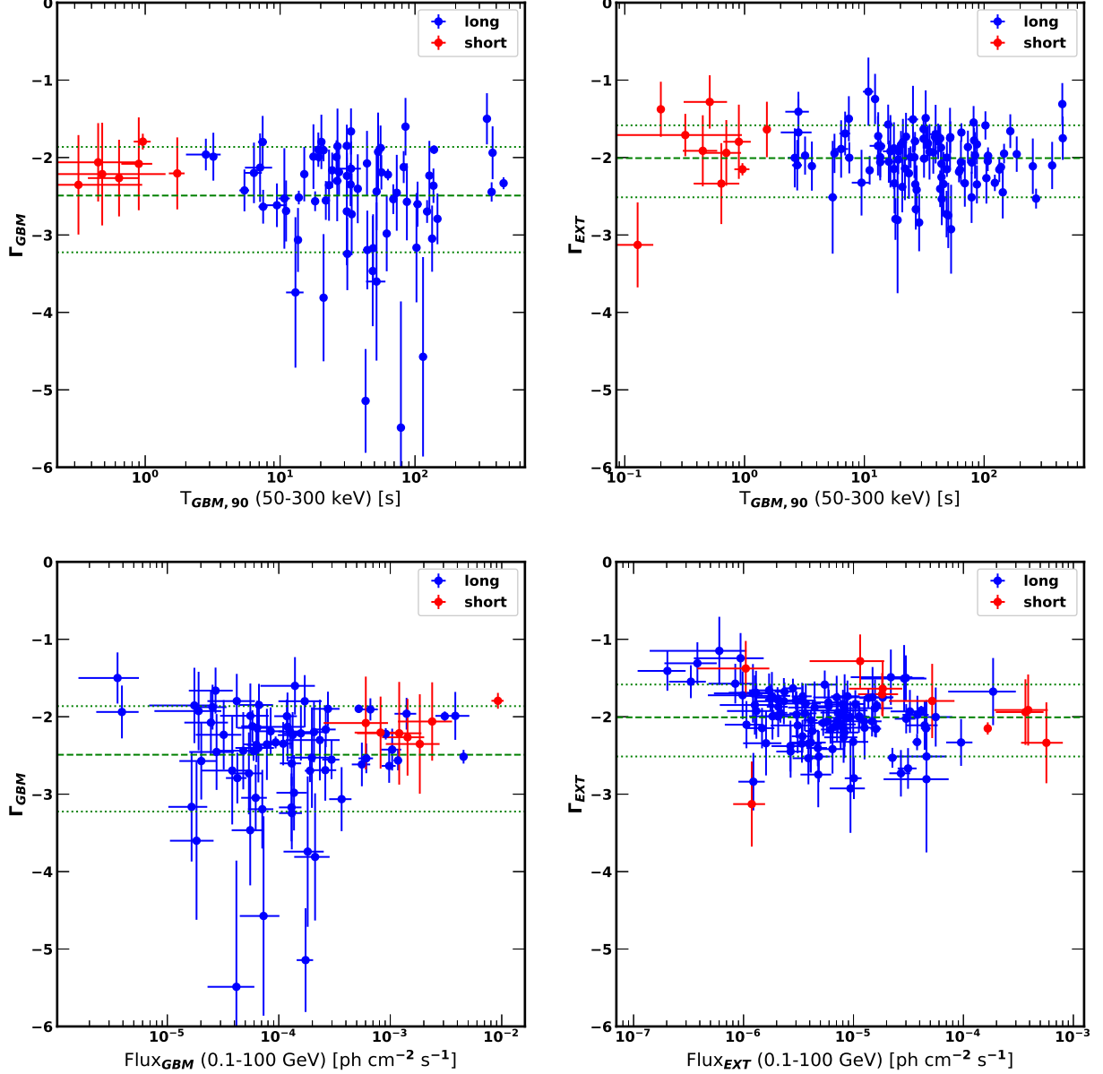
Figure 16. Photon indexes \Gamma_{GBM} (left panels) and \Gamma_{EXT} (right panels) calculated in the 100 MeV–100 GeV energy range vs. duration calculated in the 50–300 keV energy range (top panels) and LAT 100 MeV–100 GeV fluxes (bottom panels). These are calculated in the “GBM” (bottom left) and “EXT” (bottom right) time windows, respectively. The green dashed lines denote the mean values and the dotted lines the 10 % and 90 % percentile of each distribution. Blue and red circles represent long and short GRBs, respectively.
