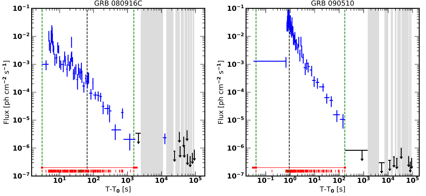
Figure 3. Temporal extended emission for two bright LAT GRBs, the long GRB 080916C ( left panel ), and the short GRB 090510 ( right panel ). Blue points show the flux in each time bin, while black arrows mark upper limits. The green vertical dashed lines indicate the first and the last LAT-detected event, while the vertical dashed black line marks the end of the GBM emission ( T_{\text{GBM},95} ). Shaded grey areas mark intervals when the GRB is outside the FoV. The red vertical markers at the bottom of each panel indicate the arrival times of the events with probability >0.9 to be associated with the GRB, with the green cross being the event with maximum energy. The horizontal red line indicates the estimated duration of the GRB ( T_{\text{LAT},100} ).
