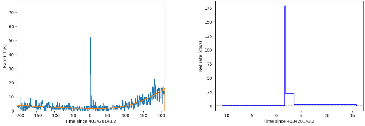
Figure 2. Left panel: LLE light curve of GRB 131014 in the 30 MeV – 1 GeV energy range. The polynomial fit to the background is marked by a red line. Right panel: Bayesian Blocks representation of the light curve of GRB 131014. All light curves are centered around the GBM trigger time T_0 = 403420143.2 (in MET).
