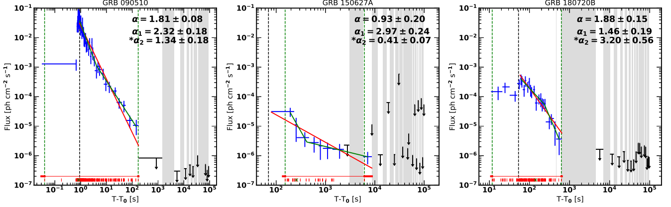
Figure 20. Temporally extended emission for three GRBs that are best fit by a BPL model (a fourth one, GRB 130427A, is shown in the left panel of Figure 9). GRB names are shown in the title in each panel. The red vertical markers indicate the arrival times of the events with probability >0.9 to be associated with the GRB, with the green cross being the event with maximum energy. The green vertical dashed lines indicate the first and the last event. The vertical dashed black line marks the T_{\text{GBM},95} . The PL and BPL fits are indicated with solid red and green lines, respectively. Fit parameters are given in the top right corner of each panel. The asterisk highlights the value selected as temporal decay index in the analysis (which, in these cases, always corresponds to \alpha_2 of the BPL model).
