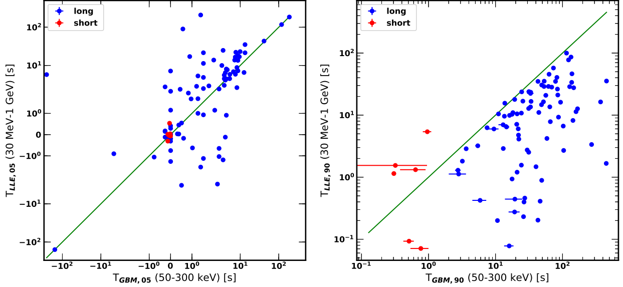
Figure 12. Onset times ( T_{LLE,05} ; left panel) and durations ( T_{LLE,90} ; right panel) calculated using LLE data in the 30 MeV–1 GeV energy range vs. the corresponding quantities ( T_{GBM,05} and T_{GBM,90} ) calculated using GBM data in the 50–300 keV energy range. The solid green line denotes where value are equal. Blue and red circles represent long and short GRBs, respectively.
