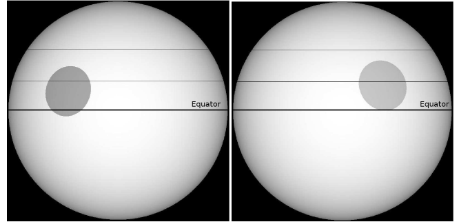
Figure 5. Representation of the stellar disc, starspot, transit chord and equator for the two datasets of WASP-6 containing spot anomalies. The axis of stellar rotation lies in the plane of the page and in the case of \lambda = 0^\circ points upwards.
