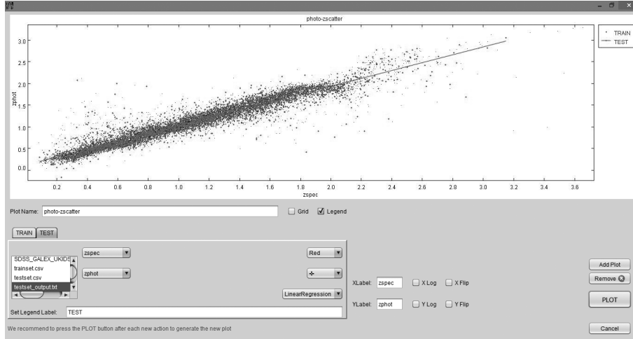
Fig. 11 The photo-z vs zspect plot as produced after a photo-z regression experiment. In this example the diagram shows both training (black dots) and test (gray crosses) objects, although the blind test objects are the most relevant to evaluate the prediction performances.
