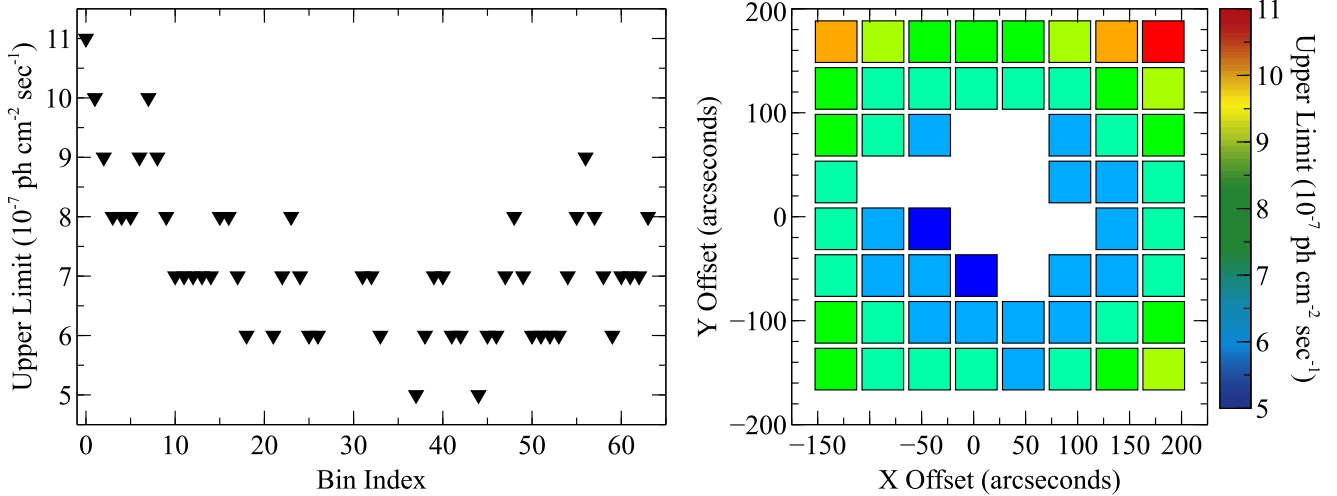
Figure 7. The upper limits for each region where the ^{44}\text{Ti} is not detected (left) and the spatial distribution of the upper limits (right). Regions where the ^{44}\text{Ti} is detected are intentionally left blank. See the text for details.
