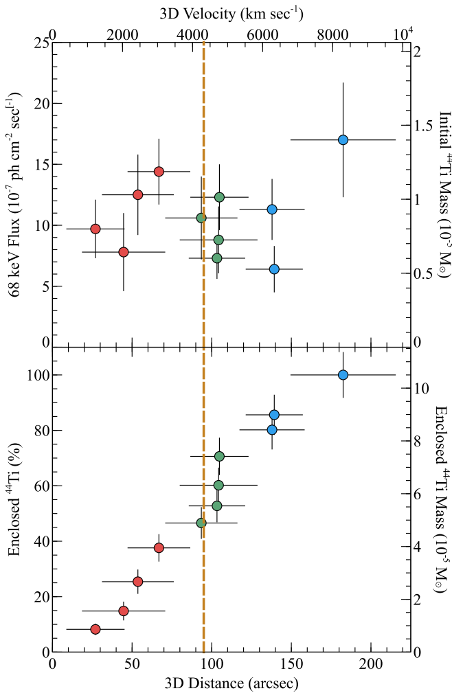
Figure 6. (Top) The flux in the 68 keV line (Y-axis) for each region is plotted against the 3D space velocity of each region (X-axis). The secondary Y-axis (right) shows the inferred initial mass of ^{44}\text{Ti} for each region assuming the distance and age of the remnant given in the text. (Bottom) The enclosed flux/mass fraction as a function of radius. Roughly 40% of the ^{44}\text{Ti} is clearly interior to the reverse shock, while 40% of the mass is at or near the reverse shock radius, leaving roughly 20% of the mass clearly exterior to the reverse shock. The color coding is the same as for Figure 4.
