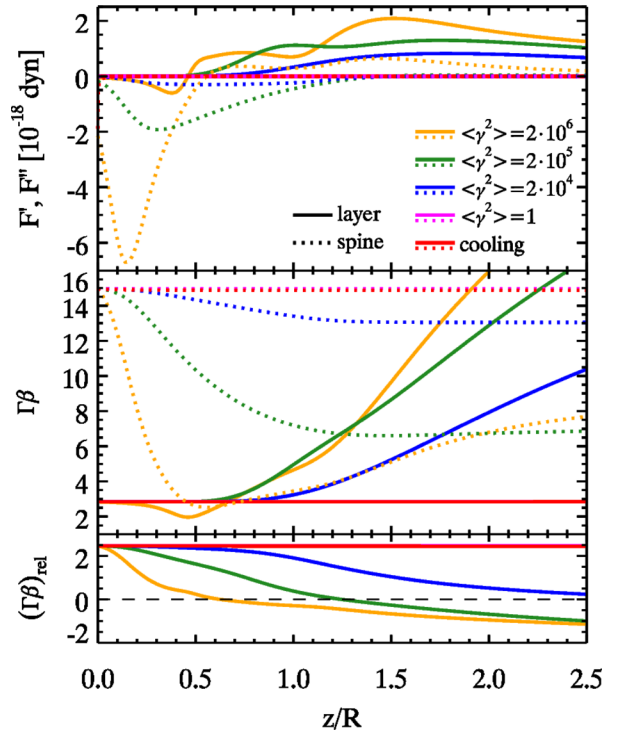
Figure 12. Radiative acceleration of the spine and the layer: the feedback. Comparison by varying \langle \gamma^2 \rangle = 2 \times 10^6, 2 \times 10^5, 2 \times 10^4, 1 of both the spine and the layer in no cooling case and cooling case. Parameters used: \Gamma_{S,0} = 15 , \Gamma_{L,0} = 3 and L_S'' = 10L_L' . Top panel: radiative force measured in spine (layer) frame in dotted (solid) lines as a function of z/R . Middle panel: profile of (\Gamma\beta) of the spine (layer) in dotted (solid) lines. Only for \langle \gamma^2 \rangle = 2 \times 10^6 with no cooling, in the final stages the layer can travel faster than the spine. Bottom panel: the relative velocity profile of the spine with respect to the layer expressed in terms of (\Gamma\beta)_{\text{rel}} .
