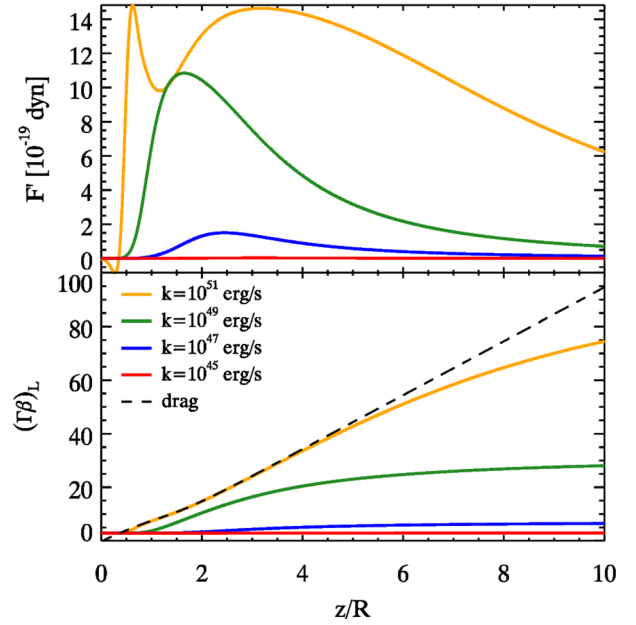
Figure 3. Radiative acceleration of the layer by varying k_L = L_{iso,S} \langle \gamma_L^2 \rangle (values from 10^{45} to 10^{51} erg s ^{-1} ). The spine Lorentz factor is constant \Gamma_S = 15 . The initial Lorentz factor of the layer is \Gamma_{L,0} = 3 . The x -axis is common for the two panels and depicts the position z normalized by the vertical structure dimension R . Top panel: radiative force F' as measured in the frame of the layer as a function of z/R . Bottom panel: layer Lorentz factor (\Gamma\beta)_L (solid lines) and the drag Lorentz factor (\Gamma\beta)_{L,drag} of the layer (dashed line) as a function of z/R .
