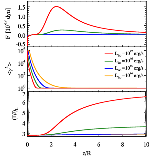
Figure 8. Radiative acceleration of the sheath obtained by varying the isotropic spine luminosity L_{\text{iso},S} from 10^{44} to 10^{47} \text{ erg s}^{-1} for the sheath constituted by hot leptons ( \langle \gamma_L^2 \rangle = 10^6 ), constant spine Lorentz factor of \Gamma_S = 15 and for an initial sheath Lorentz factor \Gamma_L = 3 . The x -axis depicts the position z in units of the vertical structure dimension R . The top panel depicts the radiative force measured in the layer frame. Middle panel: the internal energy of the sheath denoted by \langle \gamma_L^2 \rangle . Bottom panel: Lorentz factor of the sheath (\Gamma\beta)_L measured in the observer frame.
