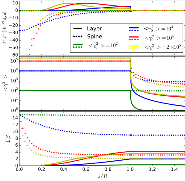
Figure 13. Radiative acceleration of the spine and the layer: the feedback with continuous injection. In this scenario, the plasma radiatively cools for z/R > 1 whereas for 0 < z/R < 1 it is continuously energized thereby nullifying the radiative cooling (thus maintaining its internal energy content). The coloured curves are obtained by varying \langle \gamma^2 \rangle = 2 \times 10^5 , 10^5 , 10^4 and 10^2 for both the spine and the layer. Parameters used: \Gamma_{S,0} = 15 , \Gamma_{L,0} = 1.01 and L_S'' = 10L_L'' . Top panel: radiative force measured in spine (layer) frame in dotted (solid) lines as a function of z/R . Middle panel: the variation in the internal energy of content of the spine and the layer denoted by \langle \gamma^2 \rangle as a function of the vertical position z . Bottom panel: (\Gamma\beta) profile measured in the observer frame.
