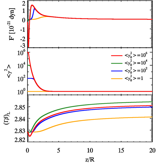
Figure 10. Same as Fig. 9, but zooming out to longer z/R to see the final values of (\Gamma\beta)_L .
