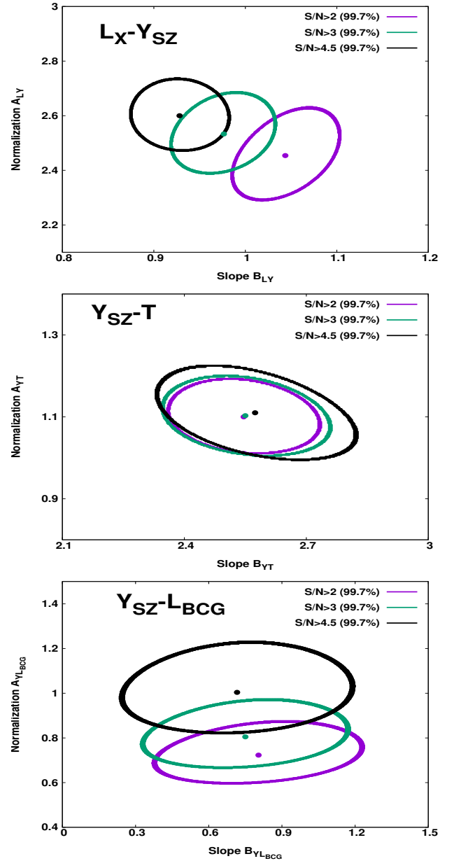
Fig. D.1. 3\sigma (99.7%) parameter space of the normalization and slope of the L_X-Y_{SZ} (top), Y_{SZ}-T (middle), and Y_{SZ}-L_{BCG} (bottom) relations for S/N > 2 (purple), S/N > 3 (green), and S/N > 4.5 (black).
