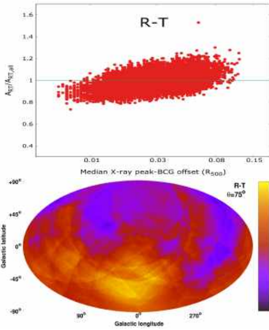
Fig. C.3. Top: correlation between the best-fit normalization A_{RT} (over the full best-fit value of the full sample) and the median XBO for every of the 10^5 bootstrap subsamples. Bottom: A_{RT} anisotropy map after calibrating for the existing correlation with the XBO.
