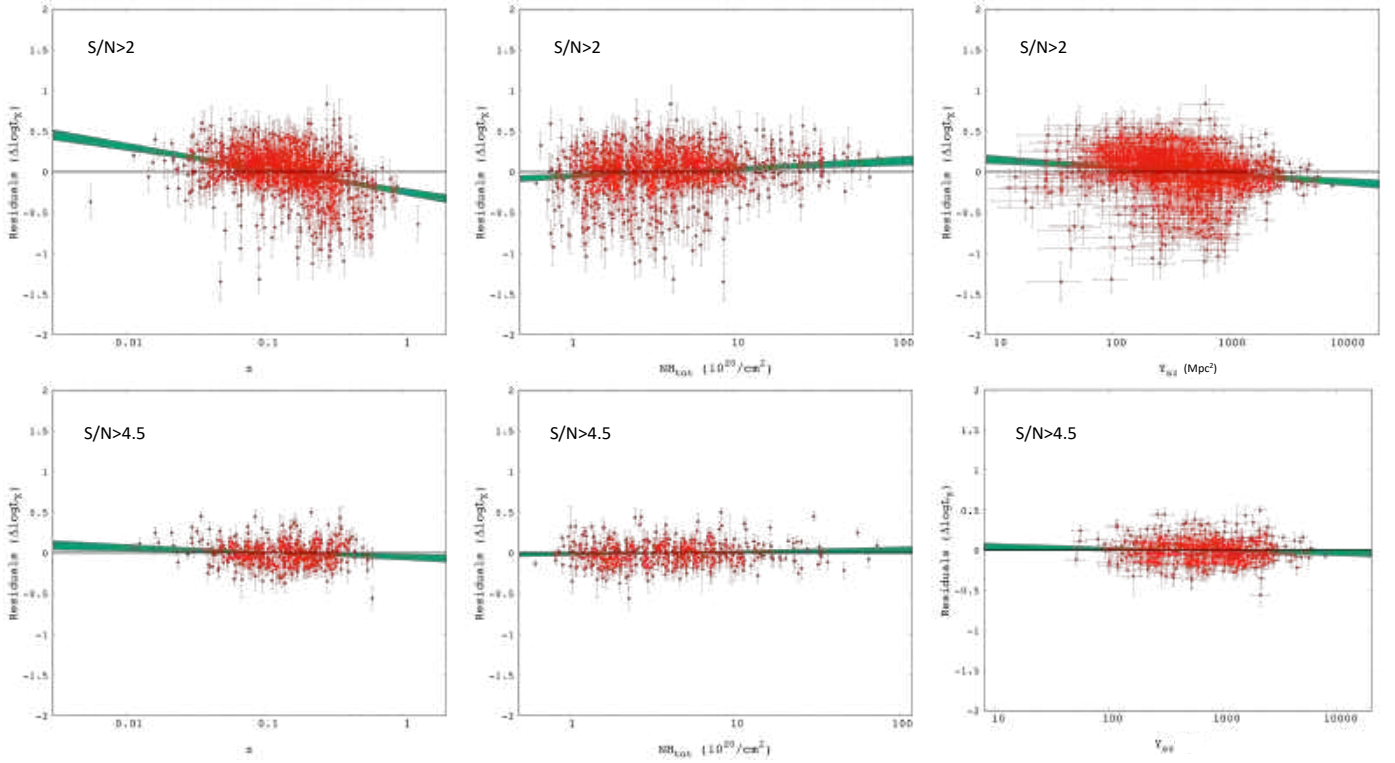
Fig. D.2. L_X residuals for the L_X – Y_{SZ} relation for S/N > 2 (top) and S/N > 4.5 (bottom) as a function of z (left), N_{H,tot} (middle), and Y_{SZ} (right). The green strips indicate the best-fit line with their 1\sigma uncertainties. It is evident that for S/N > 4.5 , the slope is always consistent with zero, indicating no dependence of the residuals on the cluster physical properties.
