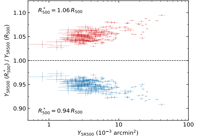
Fig. E.5. Relative change of the measured Y_{5R500} when the input R_{500} (and \theta_{500} ) is increased (red) or decreased (blue) by 6%.
