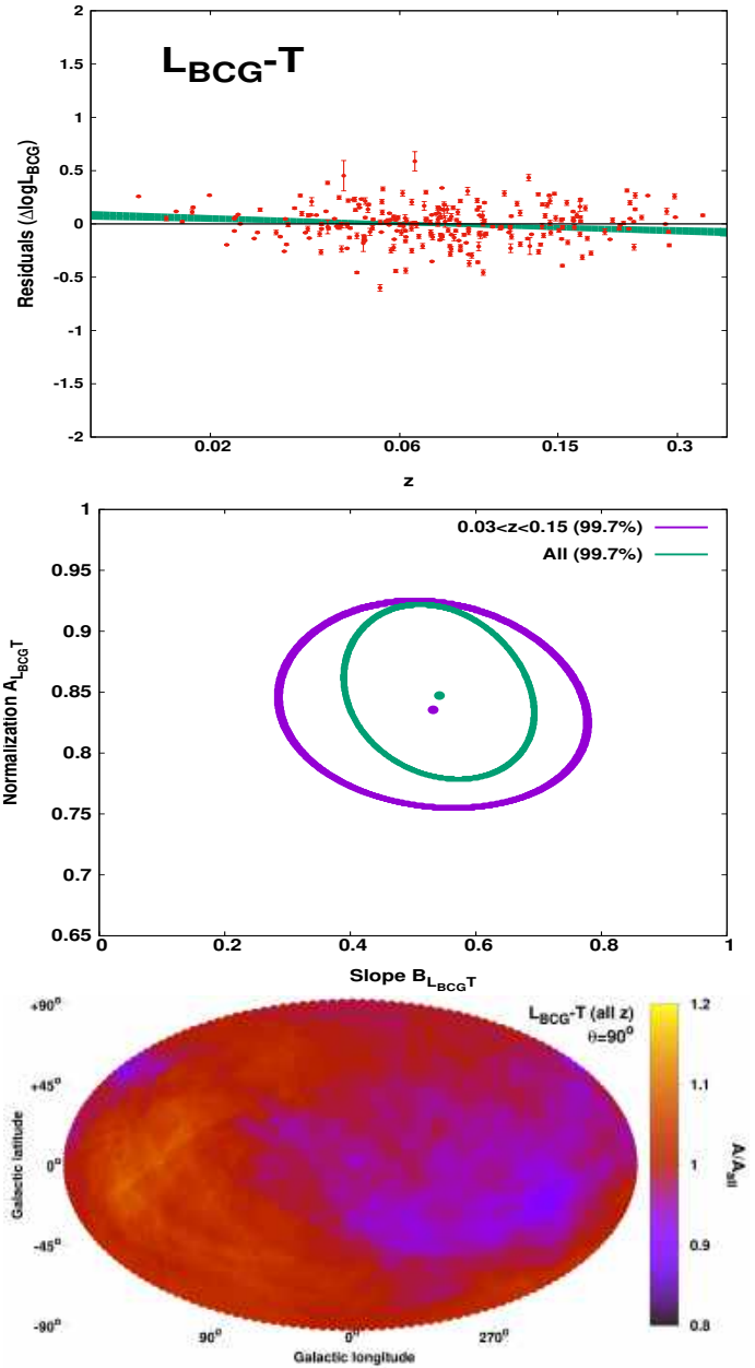
Fig. D.6. Top: L_{BCG} residuals of the L_{BCG}-T fit, as a function of the BCG redshift. The green stripe corresponds to the best-fit function within 1\sigma . Middle: 3\sigma (99.7%) parameter space of the normalization and slope of the L_{BCG}-T relation, for all clusters (green), and for 0.03 < z < 0.15 clusters (purple). Bottom: normalization anisotropy map of the L_{BCG}-T relation when all clusters are considered independent of their redshift.
