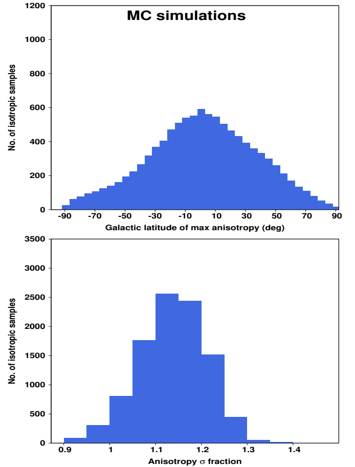
Fig. E.1. Top: distribution of the Galactic latitude of the most anisotropic regions as detected in the 10 000 isotropic simulated samples for the L_X-T relation. The distance weighting during the L_X-T fitting was used. The bins close to the ZoA cover a larger portion of the sky and naturally more anisotropies are expected to be detected there even if no bias existed.
