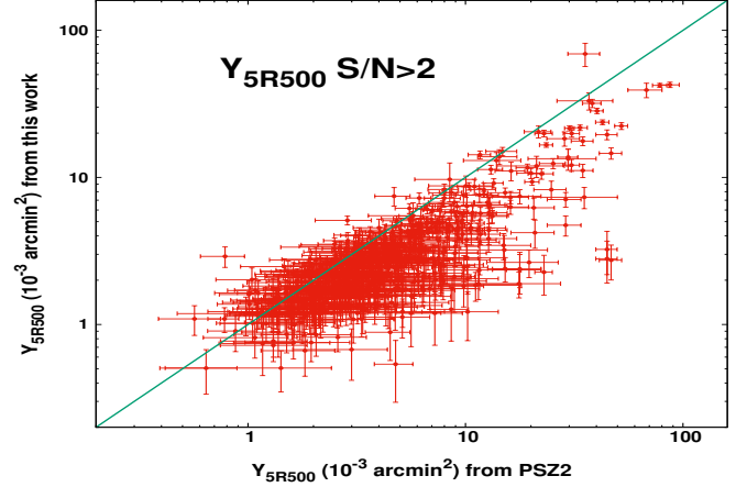
Fig. A.1. Comparison between the default Y_{5R500} values in this work based on the method of E19 and the Y_{5R500} values as given in the PSZ2 catalog for the 566 clusters in common. The equality line is shown in green.
