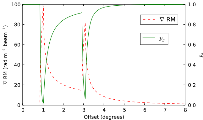
Figure 15. The depolarising effect of the spatial gradient in RM at the inner and outer edge of an ionized shell. The dotted/red line shows the gradient in rotation measure ( d\text{RM}/dr ) in units of \text{rad m}^{-2} \text{beam}^{-1} as a function of position, crossing the shell from outside to the interior. The solid/green line shows the corresponding degree of polarization calculated from Equation (17).
