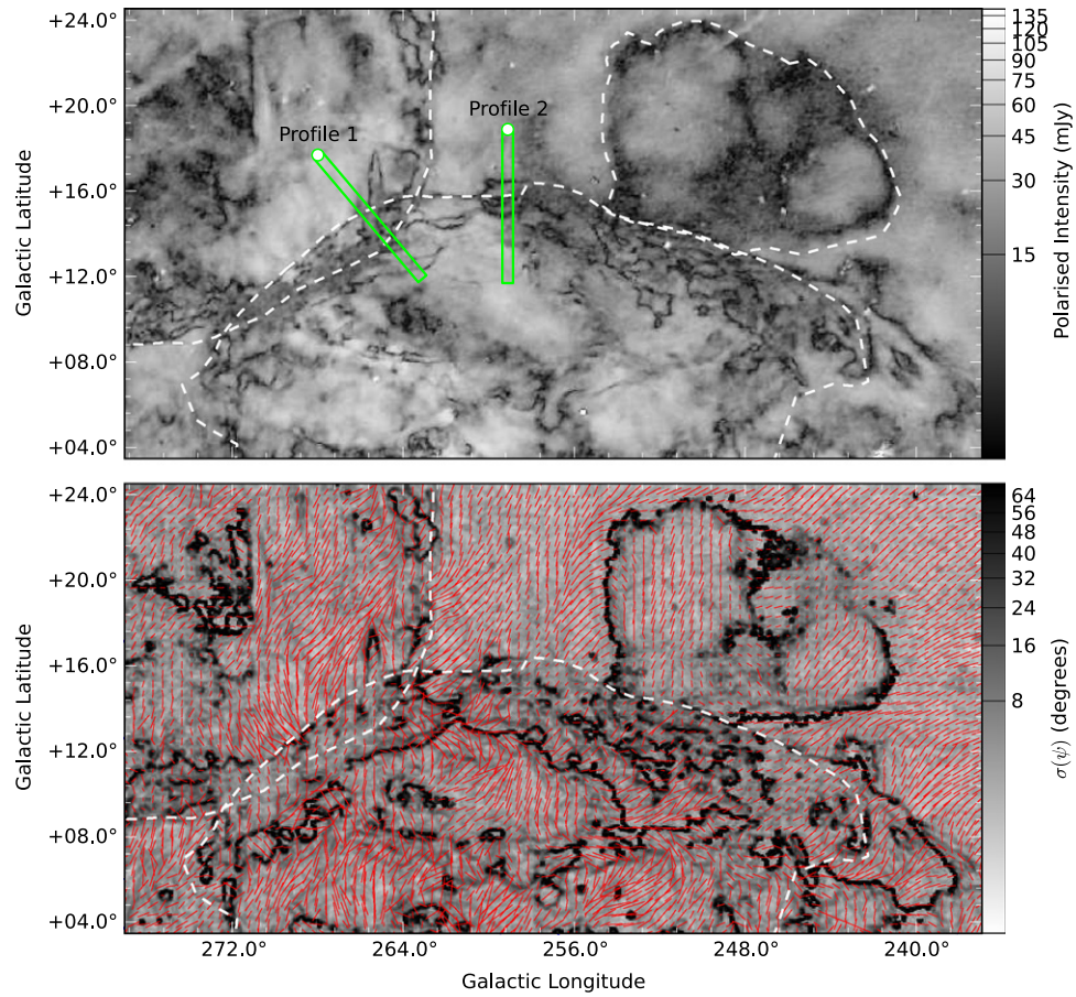
Figure 13. Top panel: map of the 2.3 GHz polarized intensity for the upper Gum Nebula. Green rectangles show where profiles have been extracted, in Figure 14 and dotted lines outline the Gum Nebula and Antlia SNR. The profiles run from (l, b) = (268^\circ 0', 17^\circ 7') to (263^\circ 1', 11^\circ 9') and (259^\circ 1', 18^\circ 9') to (259^\circ 1', 11^\circ 7') for profiles 1 and 2, respectively. Bottom panel: map of the dispersion in polarization angle \sigma(\psi) . The value of \sigma(\psi) in each pixel has been calculated from the standard deviation within a beam-sized aperture. Dark canals correspond to regions where the polarization angle varies by close to 90^\circ within a beam. The red bars over-plotted on the image every 7th pixel illustrate the orientation of the polarization vectors (magnetic vector, not corrected for RM).
