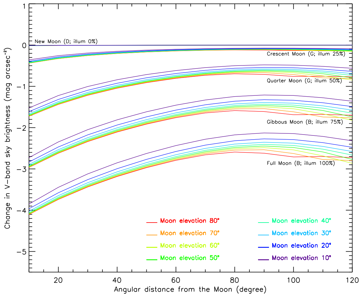
Figure 6. Change in V-band sky brightness (from dark of moon) with angular distance from the moon, for different lunar elevations (different coloured lines on each plot) and different lunar phases (as labelled).
