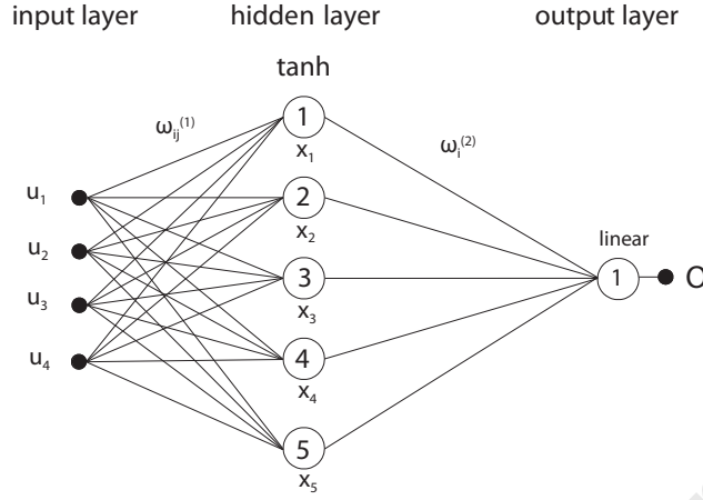
Figure 1: The scheme of the feedforward network used in the present study. The inputs u_1, u_2, u_3 and u_4 are \lambda, \phi, R_{F79} and M_a respectively. The hidden neurons have hyperbolic tangent activation functions whereas the output neuron is linear. w 's are the network weights.
