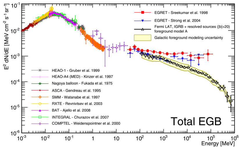
Figure 10. Comparison of the derived total EGB intensity (foreground model A) with other measurements of the X-ray and \gamma -ray background. The error bars on the LAT measurement include the statistical uncertainty and systematic uncertainties from the effective area parameterization, as well as the CR background subtraction. Statistical and systematic uncertainties have been added in quadrature. The shaded band indicates the systematic uncertainty arising from uncertainties in the Galactic foreground. (Note that the EGRET measurements shown are measurements of the IGRB. However, EGRET was more than an order of magnitude less sensitive to resolve individual sources on the sky than the Fermi LAT.)
