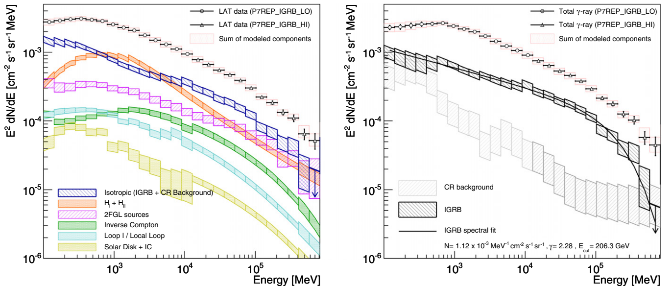
Figure 5. Results of the IGRB fit for foreground model B. See Figure 4 for legend.
