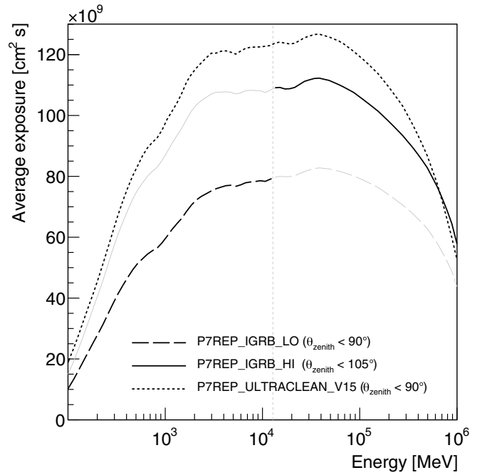
Figure 1. Comparison of the sky-averaged exposure for the P7REP_IGRB_LO, P7REP_IGRB_HI, and P7ULTRACLEAN event selections. Thick lines indicate the respective energy ranges for which the P7REP_IGRB_LO and P7REP_IGRB_HI event classes are used in this analysis.
