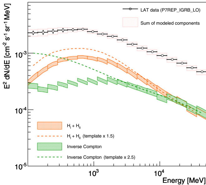
Figure 18. Fitted average intensity of the DGE in foreground model C. See Figure 14 for a description.
