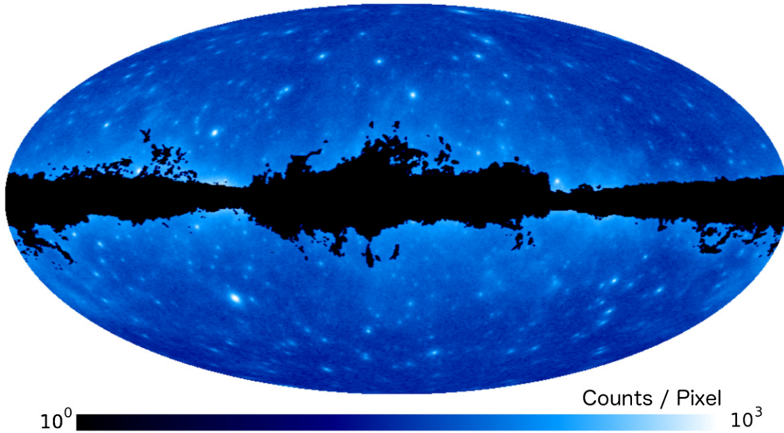
Figure 3. Map of counts observed by the Fermi LAT above 100 MeV using a Mollweide projection in Galactic coordinates with a pixel scale of \approx 0^\circ.9 . The color scale is logarithmic. Overlaid is the mask used in this analysis to exclude regions from the template-fitting procedure (see Appendix C for details).
