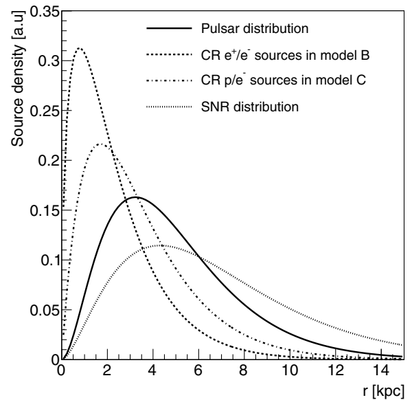
Figure 13. Parameterizations of the radial CR source distribution used in this work. The pulsar distribution is taken from Lorimer et al. (2006), the SNR distribution from Case & Bhattacharya (1998). The curves in the figure are normalized to unit integrated source density, and the actual normalizations used in the models are derived from comparisons of predicted and measured local CR proton and electron intensities.
