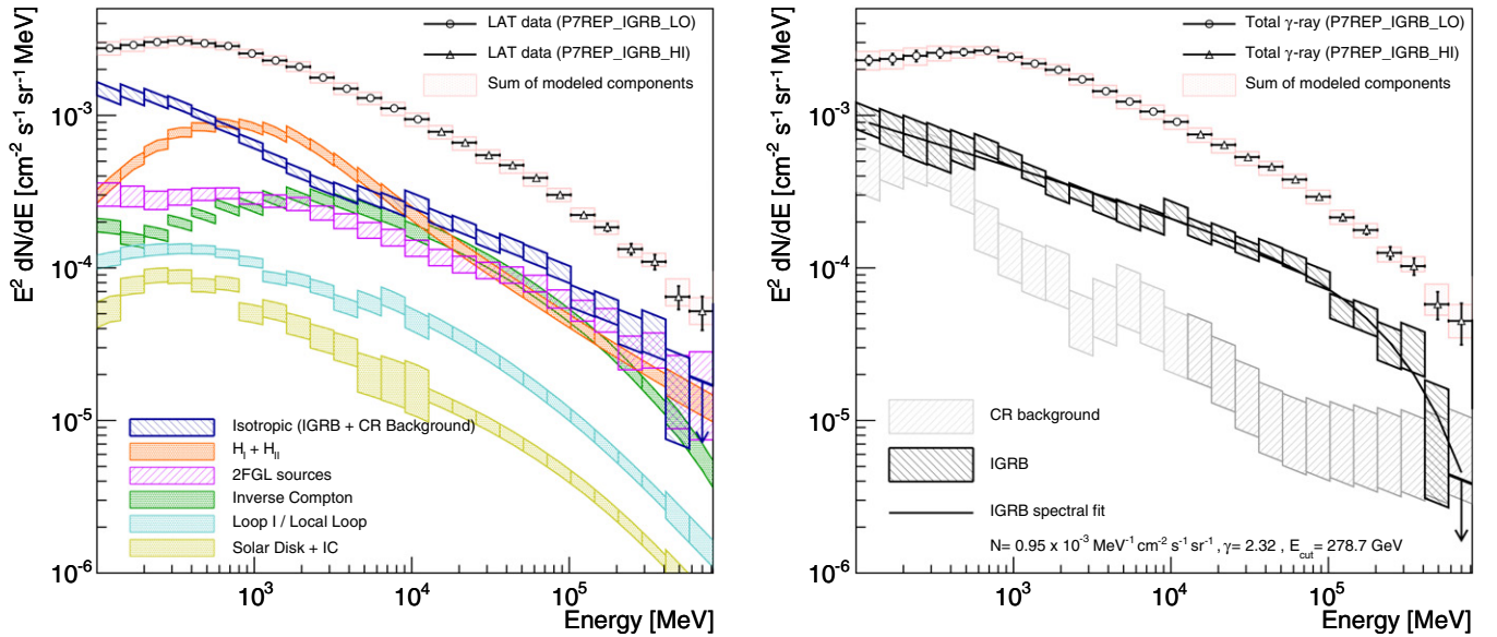
Figure 4. Results of the IGRB fit for foreground model A. Average intensities for Galactic latitudes |b| > 20^\circ are shown. Left: intensities attributed to the different foreground templates, the isotropic emission, and the individually resolved sources in the multicomponent likelihood fit. The isotropic emission and the individually resolved sources are fitted separately in each energy bin. All other components are fitted individually in each energy bin below 13 GeV and included with fixed normalizations above this energy. The total intensity obtained from the IGRB fit is compared to the total intensity observed by the LAT. Error bars include statistical errors and systematic errors from the uncertainty in the LAT effective area parameterization. See the text for details. Right: IGRB and CR background contributions to the isotropic emission. The line indicates the best-fit IGRB spectrum with a power-law plus exponential cutoff spectral model. Spectral parameters are given in the legend. The total intensities obtained from the fit and measured by the LAT are shown with the CR background contributions subtracted in this graph.
