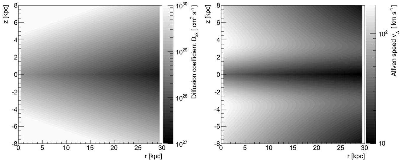
Figure 17. Diffusion coefficient (left) and Alfvén velocity (right) used in foreground model C. Both are functions of distance from the Galactic center ( r ) and height above the Galactic plane ( z ).
