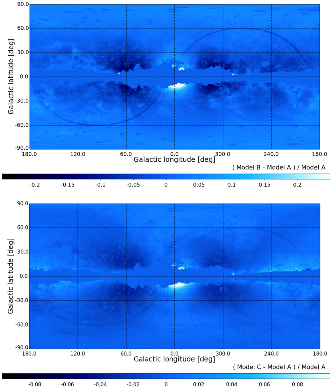
Figure 20. Differences in foreground models A, B, and C. The fractional differences in the number of predicted counts above 3 GeV between the models using the alternative Galactic foregrounds B and C and the model using Galactic foreground A are displayed in the maps. The pixel size is 0.8 \text{ deg}^2 (HEALPix order 6). Upper: fractional difference for model B. Lower: fractional difference for model C.
