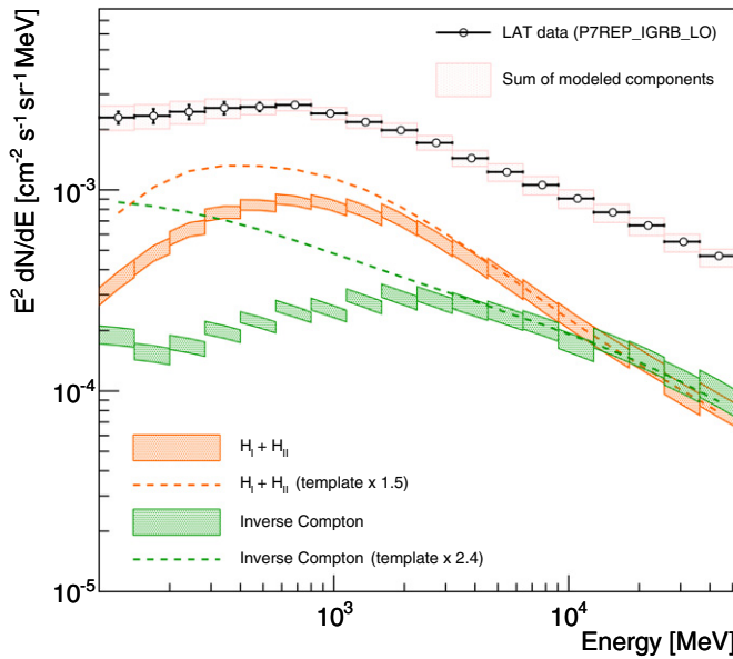
Figure 14. Fitted average intensity of the DGE in foreground model A for Galactic latitudes |b| > 20^\circ . Contributions from CR interactions with the ISG and contributions from IC are shown separately. The normalizations of the two components are fitted individually in each energy bin. The GALPROP model spectrum that enters the fit is shown as dashed lines. The dashed lines are renormalized by the factors indicated in the legend.
