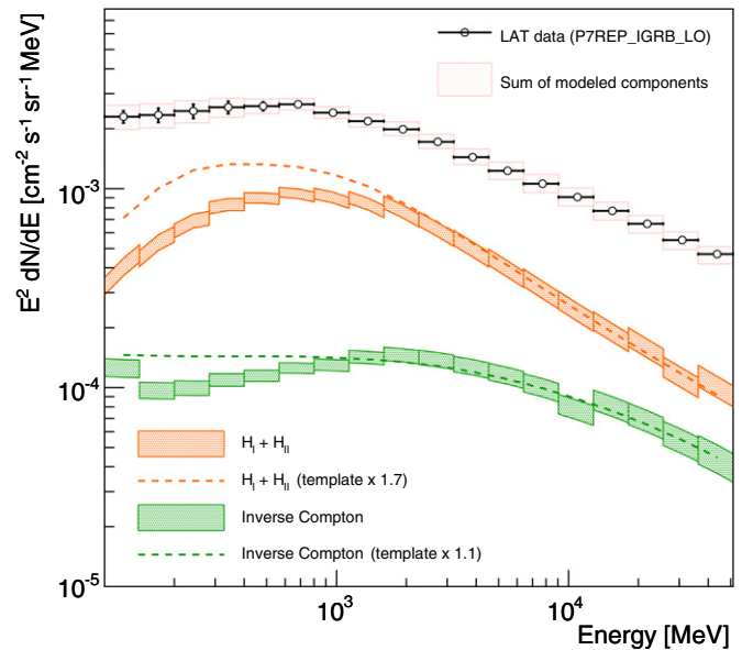
Figure 16. Fitted average intensity of the DGE in foreground model B. See Figure 14 for a description.
