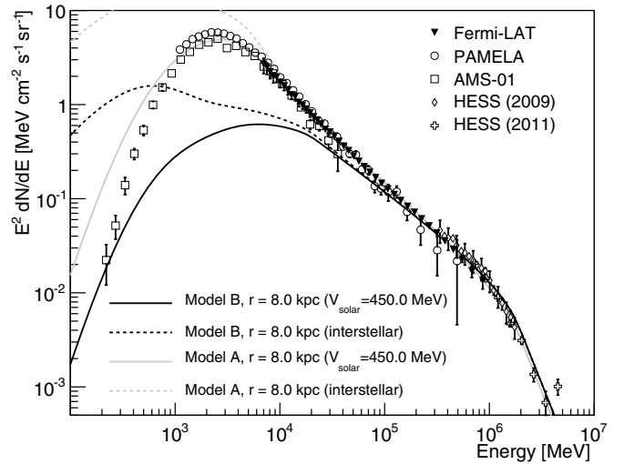
Figure 15. Predicted local CR electron spectrum of foreground models A and B in comparison to measurements of the spectrum. LAT data are taken from Ackermann et al. (2010), PAMELA data from Adriani et al. (2011a), AMS-01 data from Aguilar et al. (2002), and HESS data from Aharonian et al. (2009) and Egberts et al. (2011).
