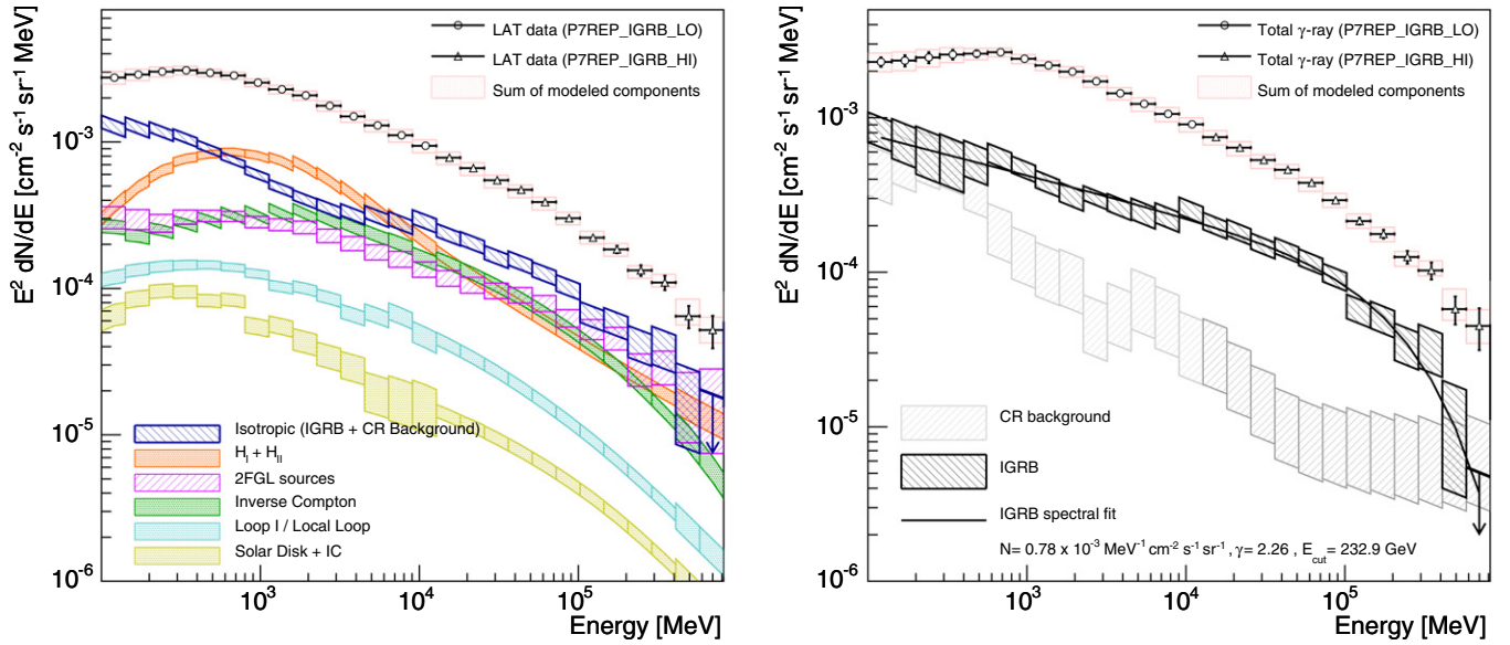
Figure 6. Results of the IGRB fit for foreground model C. See Figure 4 for legend.
