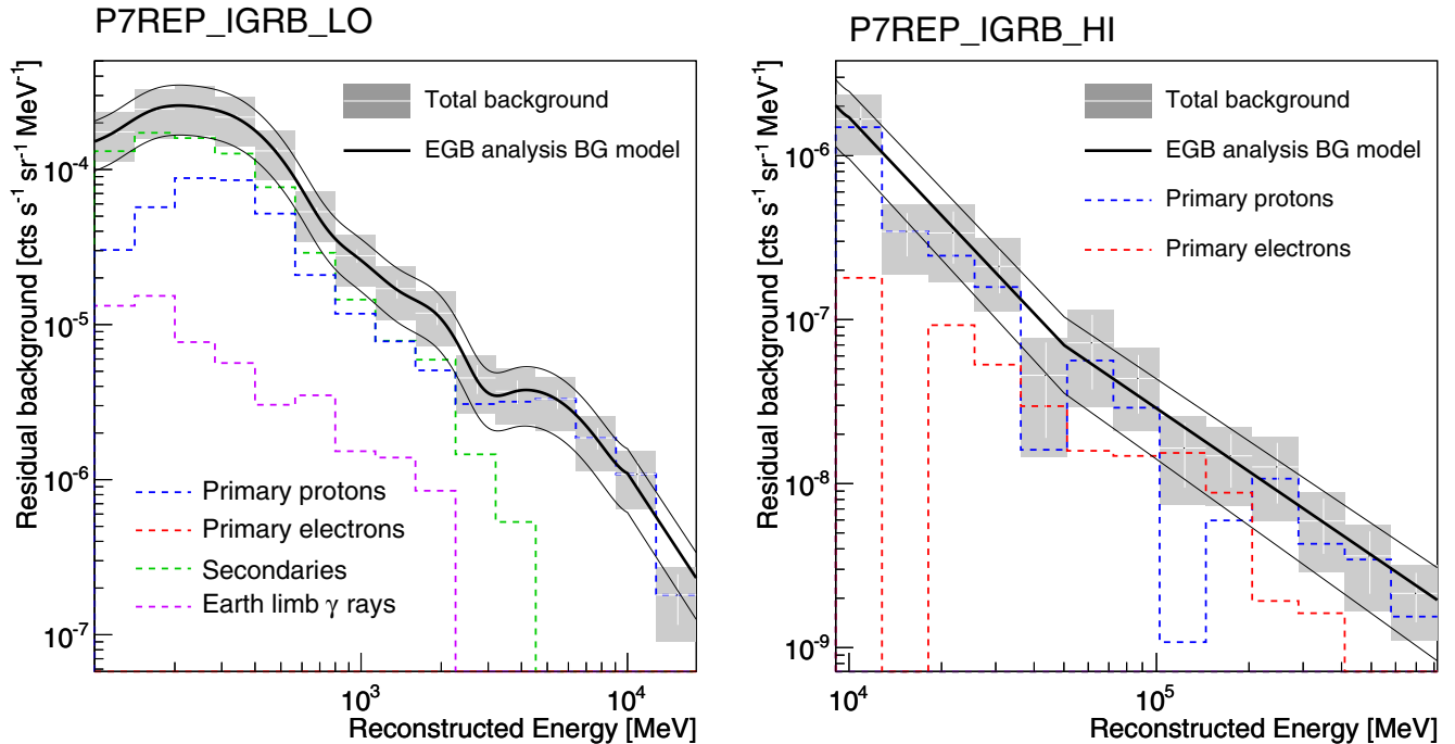
Figure 2. Comparison of the rates of residual CR background events encountered in the P7REP_IGRB_LO (left) and P7REP_IGRB_HI (right) event selections. The individual contributions from primary protons, electrons, secondary CRs, and \gamma -rays produced in the atmosphere are shown based on the respective Monte Carlo predictions. The total CR background contamination level including (gray boxes) and not including (white crosses) the systematic uncertainties is shown. A band consisting of three black lines displays the model that is used for the level (thick line) and the uncertainty (thin lines) of the CR background in the IGRB analysis.
