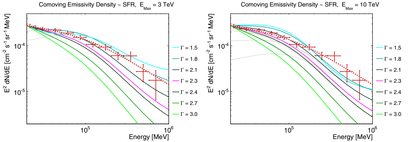
Figure 12. EGB contributions of various source population scenarios with comoving volume emissivity following the comoving star formation rate density are compared to the measured EGB spectrum (foreground model A). Each colored curve denotes a source population with a different assumed photon index. Left and right columns correspond to populations with maximum energies of 3 and 10 TeV, respectively. Gray curves represent the intensity of primary \gamma rays (attenuated by the EBL). Colored curves indicate the sum of the primary and cascade components.
