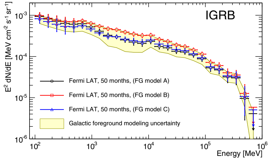
Figure 7. Comparison of the derived IGRB intensities for different foreground (FG) models. The error bars include the statistical uncertainty and systematic uncertainties from the effective area parameterization, as well as the CR background subtraction (statistical and systematic uncertainties have been added in quadrature). The shaded band indicates the systematic uncertainty arising from uncertainties in the Galactic foreground: the IGRB intensity range spanned by the three benchmark models, the variants described in Section 4.2, and the normalization uncertainties derived from the high-latitude data/model comparison. See Section 5.2 for details.
