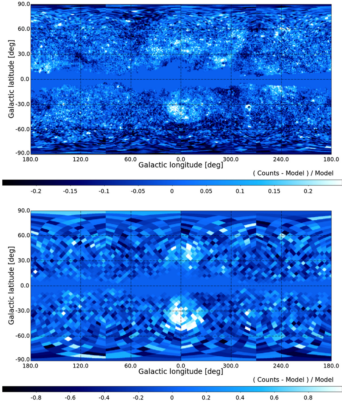
Figure 19. Residual maps for foreground model A used in this analysis. The fractional difference in counts between the actual data and the fitted model is shown in the figures. Upper: all counts above 100 MeV are included in the map. The pixel size is 0.8 \text{ deg}^2 (HEALPix order 6). Lower: only counts above 13 GeV are included in the map. The pixel size has been increased to 13 \text{ deg}^2 (HEALPix order 4) to account for the reduced count statistics at higher energies.
