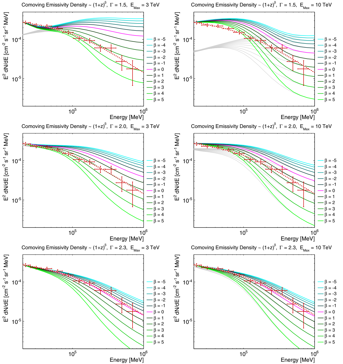
Figure 11. EGB contributions of various source populations with comoving volume emissivity parameterized by j \propto (1+z)^\beta are compared to the measured EGB spectrum (foreground model A). Rows are differentiated by the assumed photon index of the sources. Left and right columns correspond to populations with maximum energies of 3 and 10 TeV, respectively. Gray curves represent the intensity of primary \gamma rays (attenuated by the EBL). Colored curves indicate the sum of the primary and cascade components.
