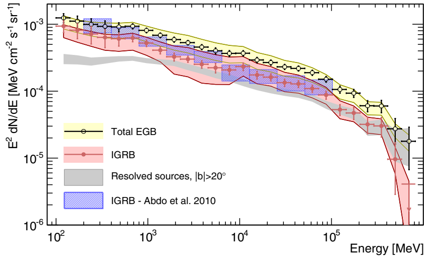
Figure 9. Comparison of the measured IGRB and total EGB intensities (foreground model A) to the first measurement of the IGRB in Abdo et al. (2010b) based on 10 months of LAT data. The error bars on the LAT measurements include the statistical uncertainty and systematic uncertainties from the effective area parameterization, as well as the CR background subtraction. Statistical and systematic uncertainties have been added in quadrature. The shaded bands indicate the systematic uncertainty arising from uncertainties in the Galactic foreground. The total EGB intensity is the sum of the IGRB and the intensity of the resolved LAT sources at high Galactic latitudes, |b| > 20^\circ .
