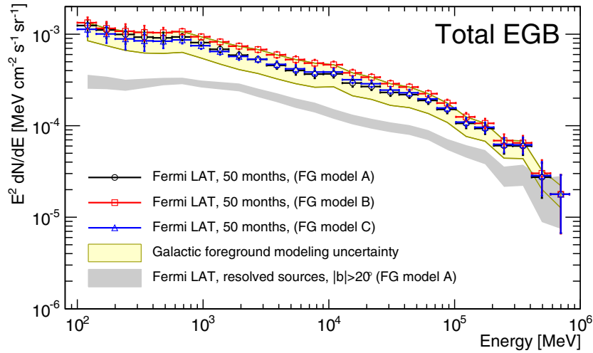
Figure 8. Comparison of the total EGB intensities for different foreground models. The total EGB intensity is obtained by summing the IGRB intensity and the cumulative intensity from resolved Fermi LAT sources at latitudes |b| > 20^\circ (gray band). See Figure 7 for legend.
