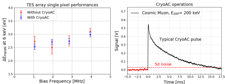
Fig. 3 TES array and CryoAC DMs operations. Left: TES array single pixel performances before and after the integration of the CryoAC in the experimental setup. Right: Typical pulse generated by a cosmic muon interacting with the CryoAC. (Color figure online)
