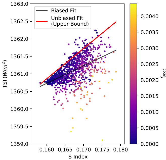
Figure 3. A plot of the SORCE TSI vs. the HARPS-N/Mt. Wilson S-index. The color of each point corresponds to the value of f_{\text{spot}} . We see that the S-index is highly correlated with the TSI, as expected. We may use this correlation to estimate the plage/network filling factors on the Sun. However, increased spot coverage results in a lower TSI value for a given S-index, which will bias our estimate of the bright region filling factor. This, in turn, will result in a less accurate estimate of the spot filling factor. The black line shows the result of the straightforward linear fit of the TSI and S-index, which is biased as described above. To isolate the plage and network-driven TSI variations, we find the 50% most densely clustered points in the above scatter plot and fit a line to the upper boundary of this region. (This choice in point density is arbitrary, but the resulting best-fit line is robust to variations in this parameter.) The resulting fit line, shown in red, is unbiased by the presence of spots.
