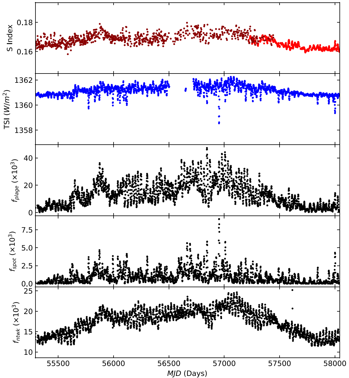
Figure 2. Time series of solar observations used in this work. From top to bottom: Mt. Wilson and HARPS-N solar telescope observations of the calcium S-index (red); Total Solar Irradiance (TSI) from SORCE/TIM (blue); and SDO/HMI plage, spot, and network filling factors (black). Note the consistent overall shapes of the S-index, TSI, and bright filling factors, and that dips in the TSI are coincident with peaks in the spot filling factor. Observations are taken between 2010 April through 2017 October. Note the two different reds used in the S-index plot: the darker red points correspond to measurements by Mt. Wilson and bright red points are from the HARPS-N solar telescope. Note that due to an instrumental anomaly, no TSI data are available from SORCE/TIM from mid-July 2013 until March 2014—we therefore do not use any times in this period in our analysis (Kopp & Lawrence 2005; Kopp et al. 2005).
