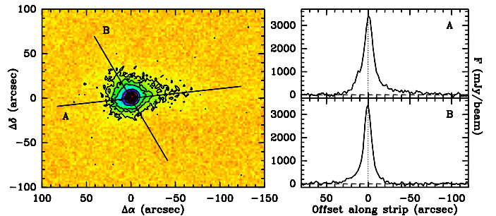
Fig. 3. SCUBA-2 map of the dust continuum emission at 450\mu\text{m} (left panel), and profiles along cuts A and B. The 450\mu\text{m} peak is at (0'', 2'') . Contours (lowest(step)highest) are 150, 300, 500(500)3500 mJy beam −1 . The rms noise is 50 mJy beam −1 .
