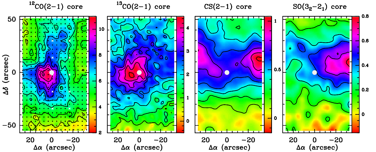
Fig. 13. IRAM data. ^{12}\text{CO} , ^{13}\text{CO} , CS, and SO \int T_A^* dv , integrated between 1.5 and 3.9 km s ^{-1} (avoiding the line wings caused by outflow). From left to right: contours low(step)max: 3(1)11 K km s ^{-1} ( ^{12}\text{CO} ); 1(0.5)4.5 K km s ^{-1} ( ^{13}\text{CO} ); 0.15(0.15)1.05 K km s ^{-1} (CS); and 0.15(0.15)0.80 K km s ^{-1} (SO). The white dot indicates the location of the 850 \mu\text{m} peak. The white crosses in the leftmost panel indicate the positions where CH _3 OH was observed. All offsets are relative to the 2MASS YSO position (see Table 1).
