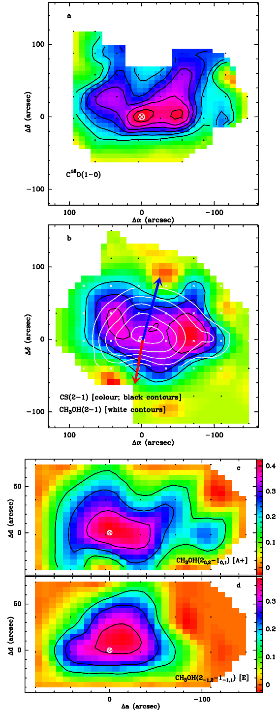
Fig. 12. Onsala data. Panel a: C 18 O(1–0) \int T_{\text{mb}} dv . Lowest contour and step: 0.6 and 0.2 \text{ K km s}^{-1} ; panel b: CS(2–1) \int T_{\text{mb}} dv (colour scale and black contours; lowest contour and step: 0.35, 0.2 \text{ K km s}^{-1} ) with CH 3 OH(2–1) \int T_{\text{mb}} dv (white contours; lowest contour and step: 0.15 \text{ K km s}^{-1} ) superimposed; the combined area under the two emission lines with the lowest upper level temperature (E and A+; Table 4 and Fig. 14) are shown. The red and blue arrows indicate the approximate direction of the outflow detected in CO(3–2) (see text). The small white crosses indicate the positions where both CS and CH 3 OH were observed; the black dots are for CS only. Panel c: CH 3 OH(2–1) \int T_{\text{mb}} dv for the A+ component (see Fig. 14) only. Lowest contour and step: 0.15, 0.1 \text{ K km s}^{-1} . Panel d: as c, but for the E-component only. In all panels, the white cross indicates the position of the 850 \mu\text{m} peak, which is also that of the embedded YSO. All offsets are relative to the 2MASS YSO position (see Table 1).
