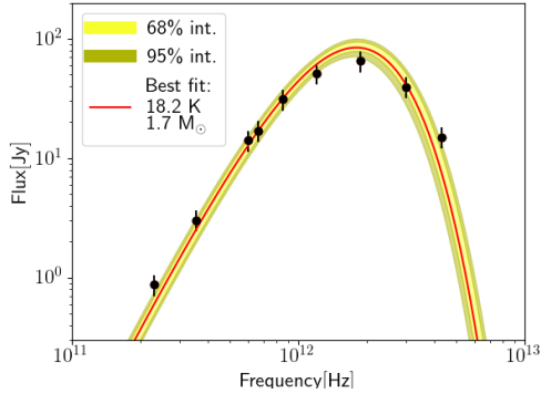
Fig. 5. Spectral energy distribution (SED) of CB230. The data shown are the SCUBA-2 measurements at 450 and 850 \mu\text{m} (corrected for CO(3–2)-emission), the integrated flux at 1.3 mm (Launhardt et al. 2010), and the Herschel data points at 70, 100, 160, 250, 350 and 500 \mu\text{m} (extracted from Fig. 4 in Launhardt et al. 2013). The fit to the data (red) was obtained by assuming a dust optical depth at 870 \mu\text{m} of 1.85 \text{ cm}^2 \text{ g}^{-1} , and a dust absorption coefficient \beta of 1.8. The yellow and green bands indicate the uncertainty in the modelled fluxes for the 68 and 95% credibility intervals of T_{\text{dust}} and M_{\text{dust}} , assuming that the uncertainty on the measured fluxes is 20%.
