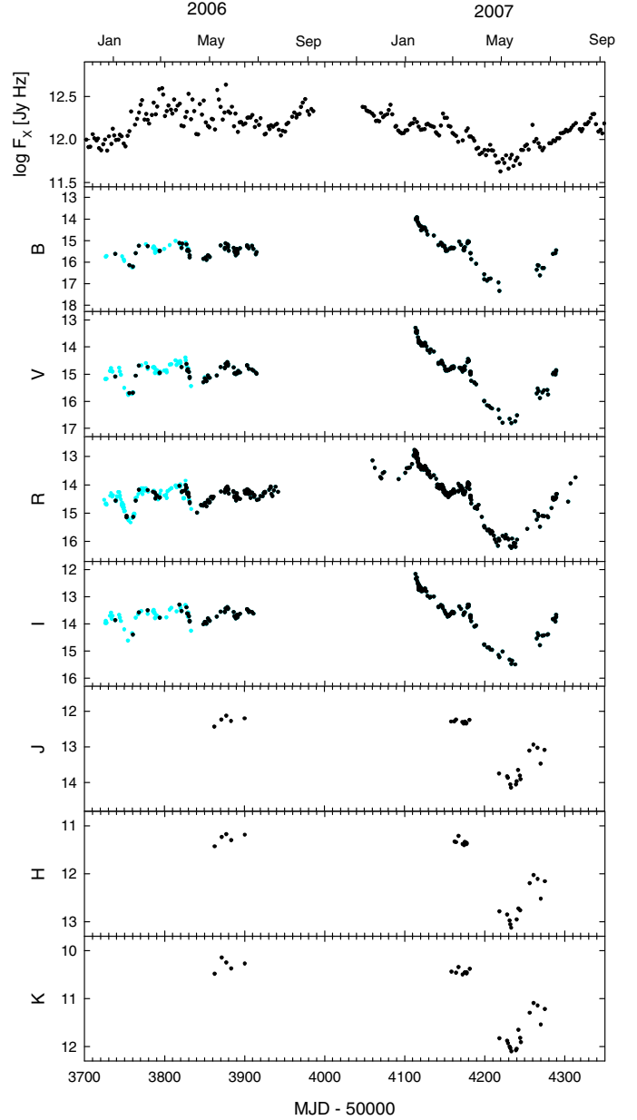
Fig. 1. X-ray, optical and near-IR light curves of 3C 279 in the 2006–2007 observing seasons. Previously published data are marked with blue (light) symbols.
