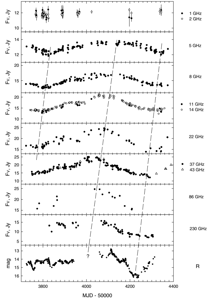
Fig. 10. Radio and R -band light curves of 3C 279; dashed slanted lines trace minima and maxima of light curves at different frequencies. Error bars are shown only for 1 and 2 GHz data, where they are larger than symbol size.
