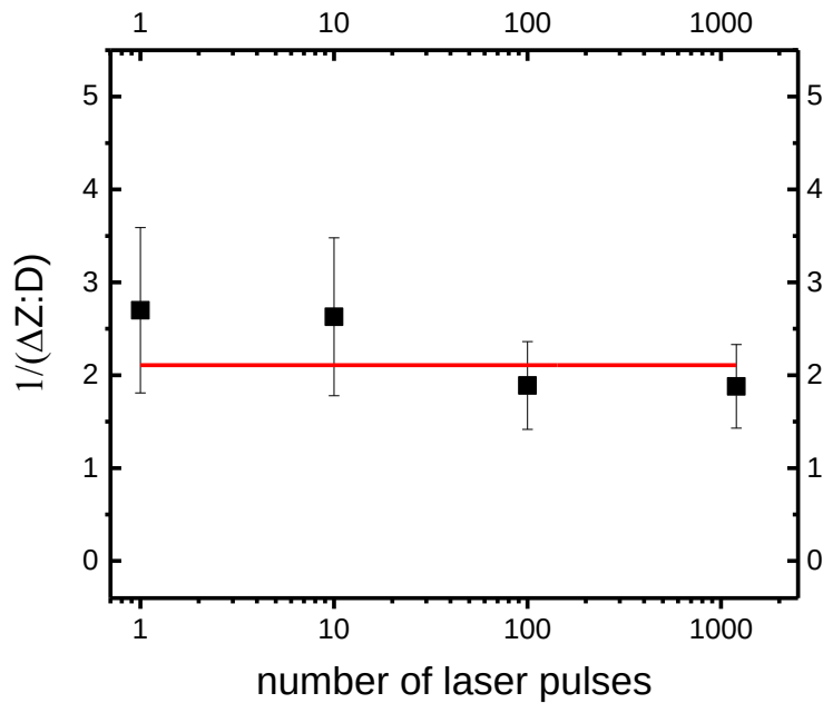
551 Figure 5: Reciprocal of the depth:diameter ratio for the impact craters formed in air on 552 the jadeite sample as a function of the total number of laser pulses: 1, 10, 100, and 1200 553 pulses. For all experiments E_{pulse} and F_{pulse} have been kept fixed and equal to 6 mJ and 554 4.2 J/cm 2 , respectively. To guide the reader's eye, the intercept y=2.1 (discretionally 555 chosen) is shown as a red line.
