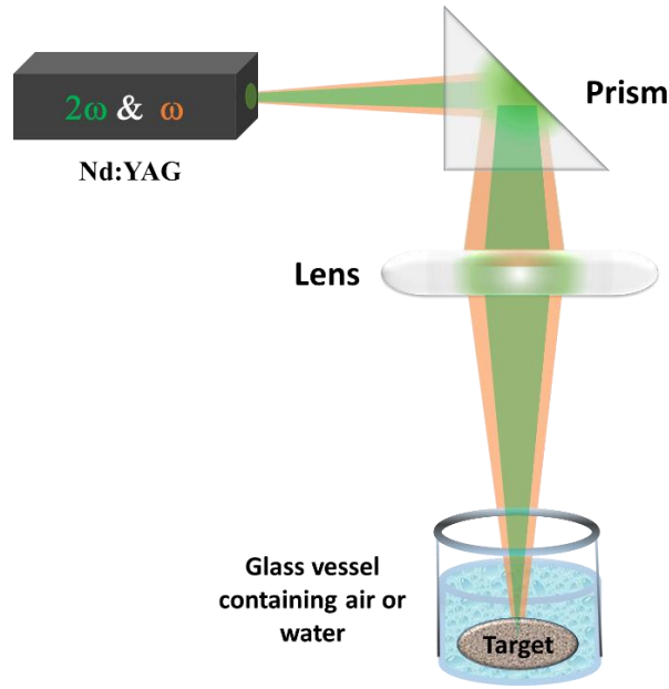
Figure 1: Schematic of the laser ablation setup used in the experiments to simulate the micrometeorite impacts. The laser source simultaneously emits pulses at both \omega and 2\omega frequency (see main text for the details).
