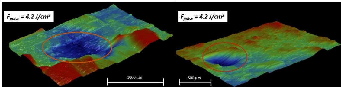
Figure 3: Crater created in the quartz sample after ablation (1200 total pulses) in deionized H 2 O with fluence 4.2 J/cm 2 (left) and after ablation in air with fluence 4.2 J/cm 2 (right). Red circles indicate crater locations.
