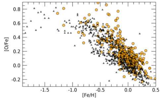
Fig. 20. Same as Fig. 17, but for [O/Fe] vs. [Fe/H] .
