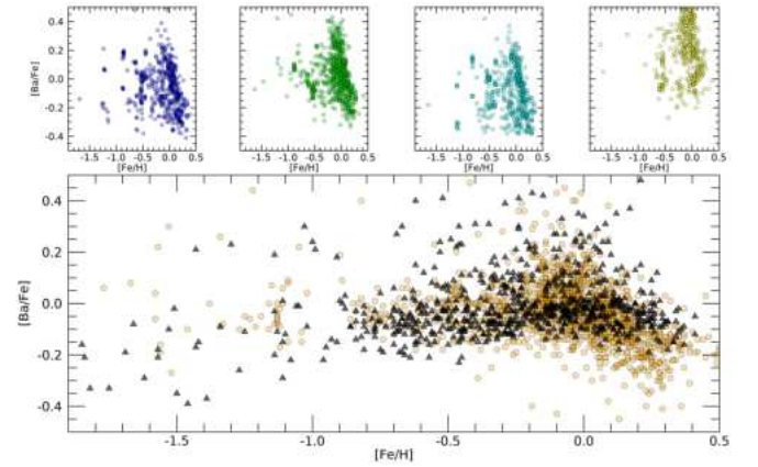
Fig. 19. Same as Fig. 17, but for [Ba/Fe] vs. [Fe/H] .
