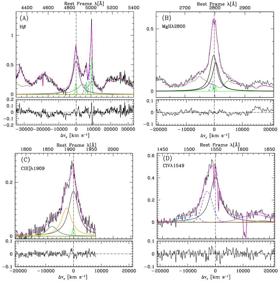
Figure 5. Multicomponent fits for 3C 57. H\beta and Mg\ II\ \lambda 2800 from CAHA spectrum and C\ III]\ \lambda 1909 and C\ IV\ \lambda 1549 from HST spectrum. The upper abscissa is rest-frame wavelength in \text{\AA} , the lower abscissa is in radial velocity units and the ordinate is specific flux per unit wavelength in arbitrary units. The vertical long dashed line indicates the adopted rest frame. The black lines show the original continuum-subtracted spectra while the dashed magenta indicates the fit to the entire spectrum. The thick black and thin green lines show the broad and narrow components, respectively. The blue-shifted component is indicated by a dashed blue line when detected. The light grey lines trace Fe\ II_{UV} and Fe\ II_{opt} emission which is considered in all four fittings. In some of them (as H\beta and Mg\ II\ \lambda 2800 ), the contribution is very important but in others (as C\ III]\ \lambda 1909 and C\ IV\ \lambda 1549 ) it is negligible. In panel (C), apart of C\ III]\ \lambda 1909 we show Si\ III]\ \lambda 1892 , Al\ III\ \lambda 1860 and Si\ II\ \lambda 1814 in orange, dark green and yellow, respectively. In panel (D), together with C\ IV\ \lambda 1549 we plot the N\ IV]\ \lambda 1486 component in cyan and the He\ II\ \lambda 1640 broad and blue component in brown and violet, respectively.
