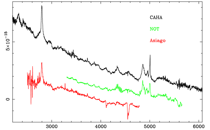
Figure 3. New spectra for 3C 57 covering Mg II \lambda 2800 and H \beta in the rest frame. Abscissa is wavelength in Å and ordinate corresponds to specific flux in units of erg s -1 cm -2 Å -1 . NOT and Asiago spectra have been vertically displaced by -1 \times 10^{-15} and -2 \times 10^{-15} erg s -1 cm -2 , respectively for presentation.
