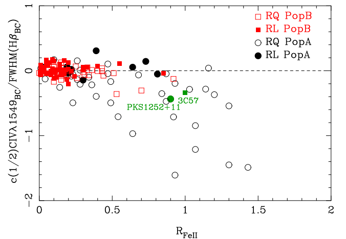
Figure 2. Location of 3C 57 and PKS 1252+11 in a 4DE1 UV-optical plane defined by normalized \text{FWHM } \text{CIV } \lambda 1549 versus R_{\text{FeII}} . RL and RQ sources are marked as filled and open symbols, respectively. Pop A sources are represented by black circles while Pop B by red squares.
