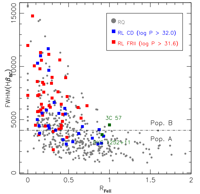
Figure 1. Location of 3C 57 in the optical plane of the 4DE1 space defined by \text{FWHM } H\beta_{\text{BC}} versus R_{\text{FeII}} . Filled red squares are LD RL sources, filled blue square CD RL sources following the definition of Z08 with weaker CD RL ( \log L_{1415\text{MHz}} < 32.0 \text{ erg s}^{-1} \text{ Hz}^{-1} ) omitted for clarity. Filled grey circles correspond to RQ quasars.
