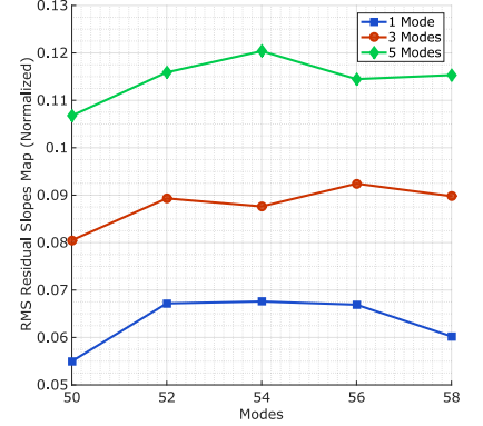
(c) Error on the Slopes Maps retrieved on-sky when modulating 1 mode ( 5 \times 500 iterations), 3 modes ( 3 \times 500 iterations) and 5 modes (500 iterations) at the same time. (5 nm RMS amplitude)
