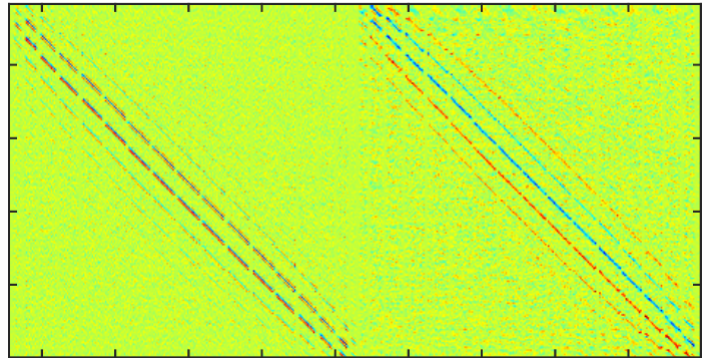
(b) Noisy zonal IM (DM Actuators \times WFS slopes) retrieved from closed-loop data (40 000 frames with \Delta T=5 )
