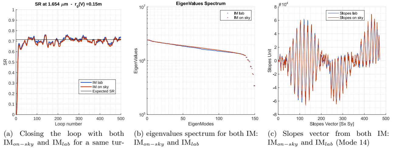
Figure 5: Validation of the on-sky calibration method using modulation signals
