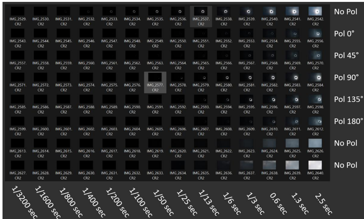
Figure 12: the full sequence of images acquired with the DSLR during the totality.
