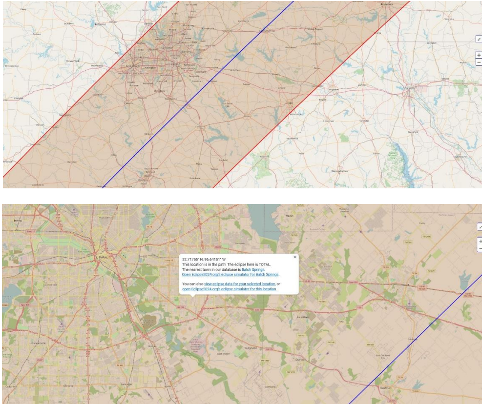
Figure 3: maps (with two different zoom) of the location chosen in Dallas TX for the 8 th April 2024 TSE observations with respect to the centre of totality (blue line) and the TSE area (red lines, provided by the “eclipse2024.org” interactive map).
