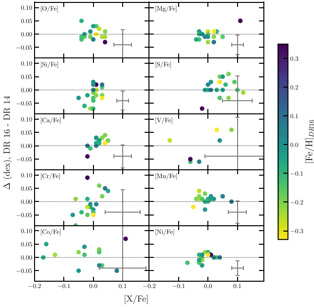
Figure 4. Similar to Figure 3, but for other elements. Characteristic error bars are shown. Data points are colored by their [\text{Fe}/\text{H}] , as reported in APOGEE DR16
