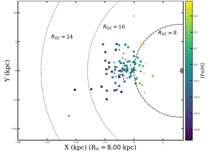
Figure 2. The full OCCAM DR16 sample plotted in the Galactic plane. Square points are “high-quality” clusters, triangles are the lower-quality clusters. The colorbar shows [Fe/H]. The concentric circles show R_{GC} = 8, 16 , & 24 kpc.
