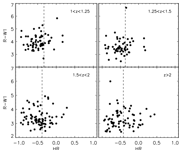
FIG. 21.— Similar to Figure 20 but for redshift ranges ( top left ) 1 < z < 1.25 , ( top right ) 1.25 < z < 1.5 , ( bottom left ) 1.5 < z < 2 , and ( bottom right ) z > 2 . Again, optical obscuration, as parameterized by R - W1 , is unrelated to X-ray absorption as implied by HR.
