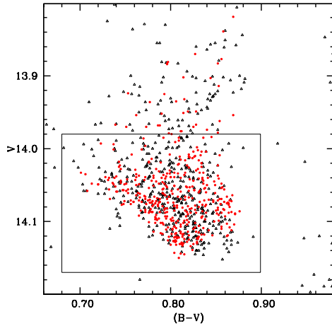
Fig. 7. A comparison between the observed HB (circles) in the GGC 47 Tuc, and a synthetic HB model obtained by assuming an uniform He distribution between Y=0.256 and 0.286 , and an average –He-independent– mass lost by the RGB progenitors equal to \Delta M \approx 0.23M_{\odot} , with a Gaussian spread by 0.005M_{\odot} .
