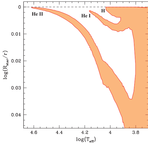
Fig. 4. The location of the convective layers associated to the H I, He I and He II ionization zones as a function of the T_{\text{eff}} ZAHB location in canonical stellar models.
