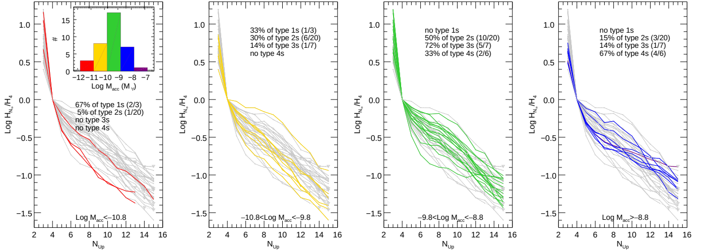
Fig. 8. Decrements and mass accretion rate. The \dot{M}_{\text{acc}} distribution histogram is shown in the first panel; the decrements relative to each bin are displayed using the same colour code as in the histogram.
