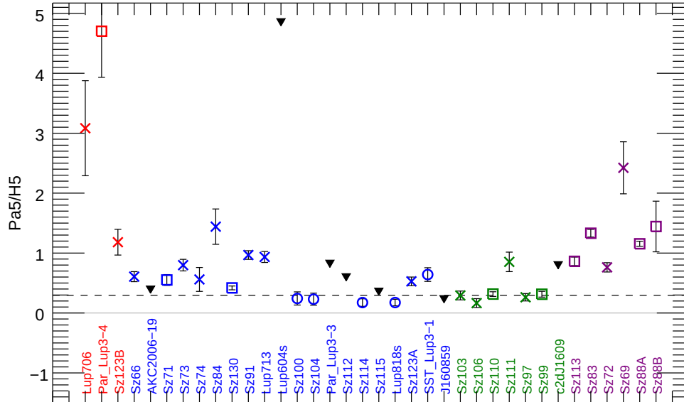
Fig. 9. Values of the Pa5/H5 ( \text{Pa}\beta/\text{H}\gamma ) in the sample. The expected value for optically thin emission is marked with a dashed horizontal line. The colour marks the decrement shape type (red:1, blue:2, green:3, purple:4) while the symbol indicates the line profile typology (circle: narrow symmetric, square: wide, cross: multi-peaked); downward triangles are upper limits.
