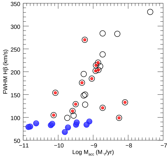
Fig. 6. FWHM of the H\beta line as a function of the \dot{M}_{acc} of the objects. The blue points indicate the narrow symmetric line sources (NS) while multi-peaked line objects (MP) are flagged with a red point. Accretion rates of the sub-luminous objects have been corrected for their obscuration factor (see Alcalá et al. 2014 and Table 1).
