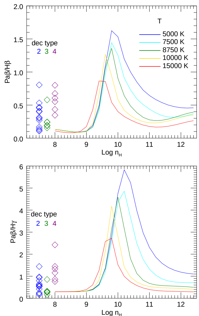
Fig. 13. Measurements of the \text{Pa}\beta/\text{H}\beta (top) and \text{Pa}\beta/\text{H}\gamma (bottom) ratios, which are displayed in the left portion of the plot and divided by Balmer decrement types (we do not include type 1 based on considerations in Sect. 4.6), are compared with KF model curves that are plotted versus the total hydrogen density for different gas temperatures (see legend in the upper panel).
