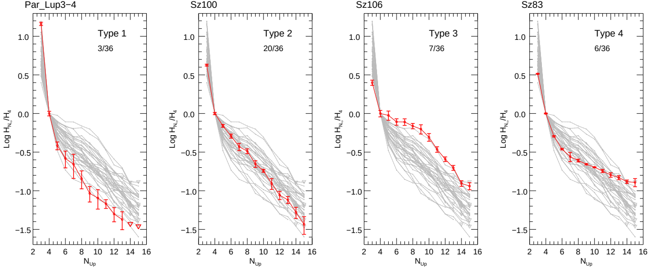
Fig. 3. Four main Balmer decrement shapes observed in our sample. From left to right: type 1 ( curved , ParLup 3-4), type 2 ( straight , Sz100), type 3 ( bumpy , Sz106), and type 4 ( L-shape , Sz83). Each type is highlighted in red against the decrements observed for all other stars (in grey).
